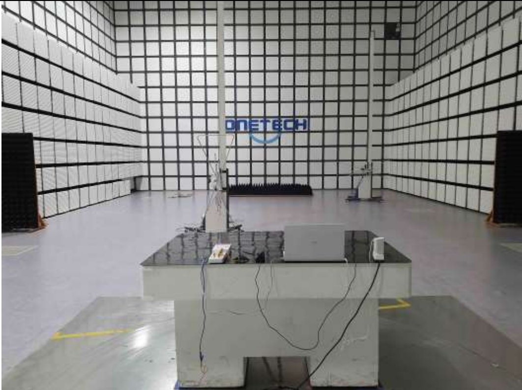
Radiated Emission
