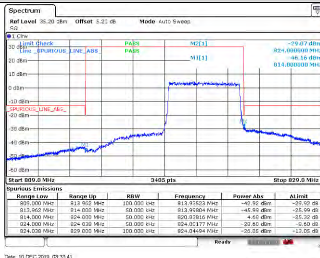
Band26-10MHz-QPSK-26740_Left-1RB#0
