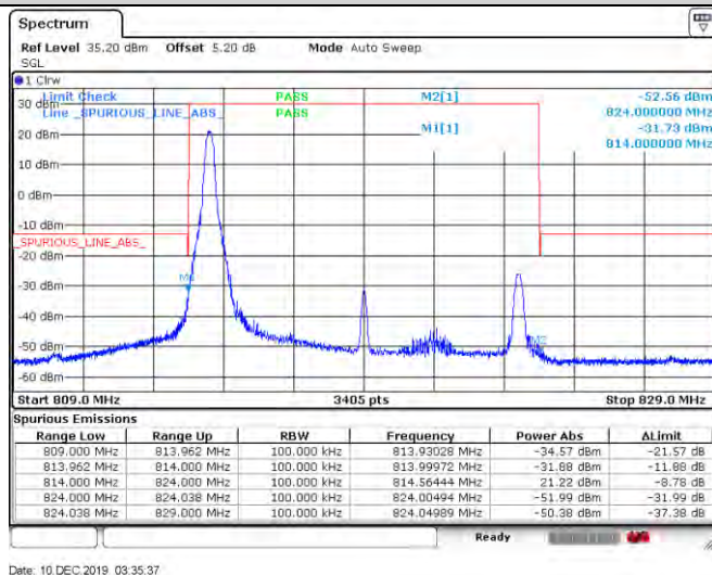
Band26-10MHz-16QAM-26740_Right-1RB#49
