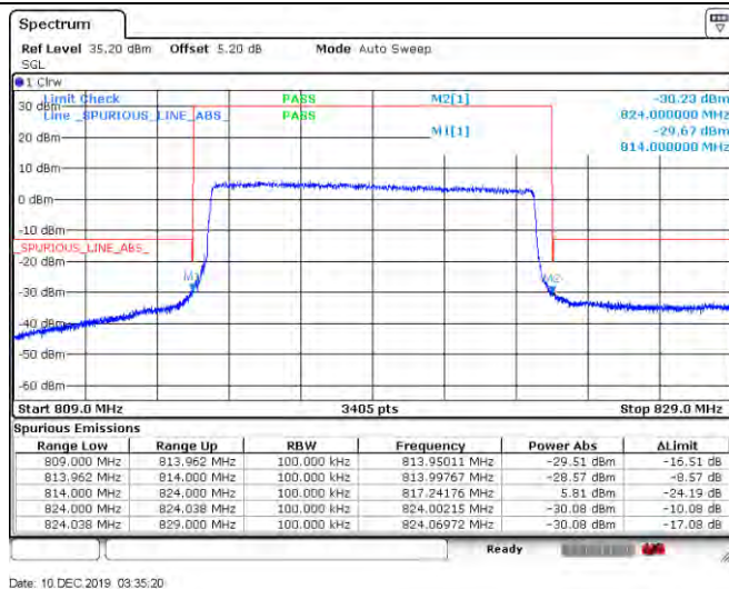
Band26-10MHz-16QAM-26740_Left-1RB#0
