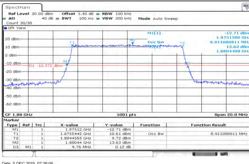
Band2-10MHz-16QAM-19150-50RB#0-8.911
