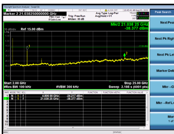
GFSK (BLE 1Mbps) LOW CHANNEL, SPURIOUS 2 GHz ~ 25 GHz
