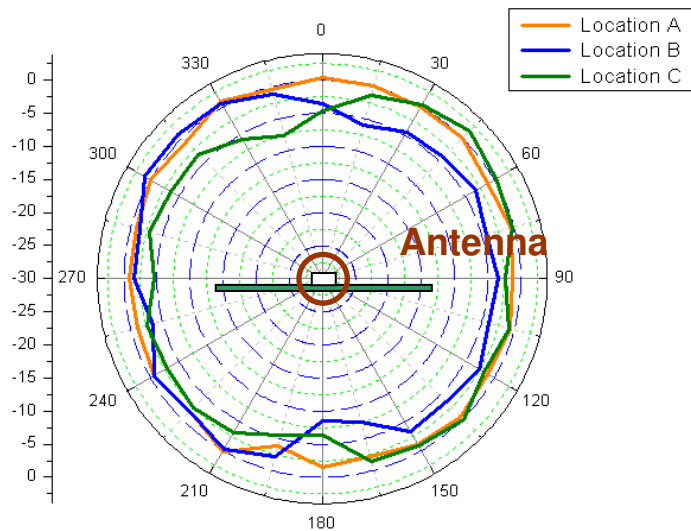
Y-Z plane 2450 MHz
