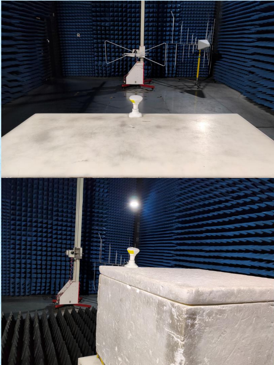
Radiated Emission
