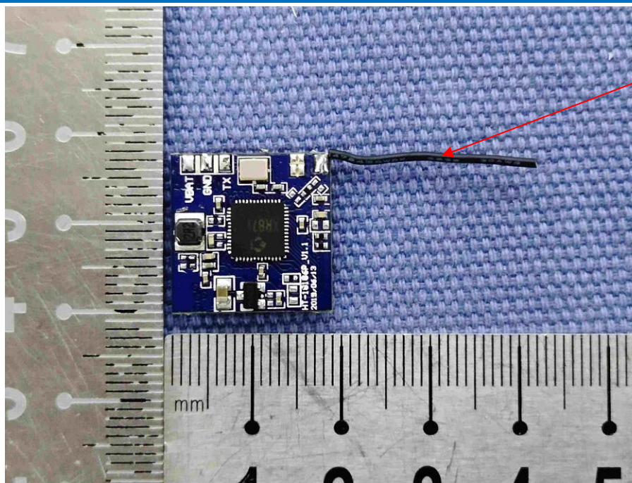
WIFI Antenna
