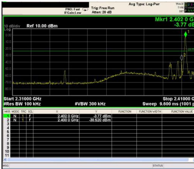
GFSK: Band Edge-Low Channel (Hopping Mode)
