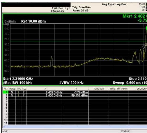
\pi/4 -DQPSK: Band Edge-Low Channel
