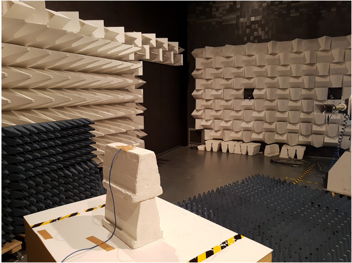
Radiated emission 1GHz - 18 GHz
