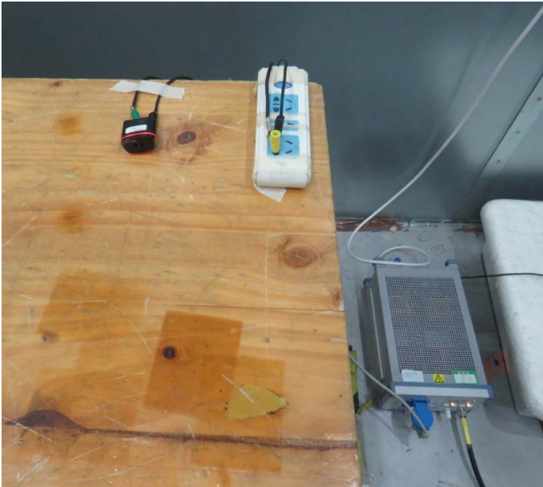
Picture 2 Conducted Emission Test Setup
