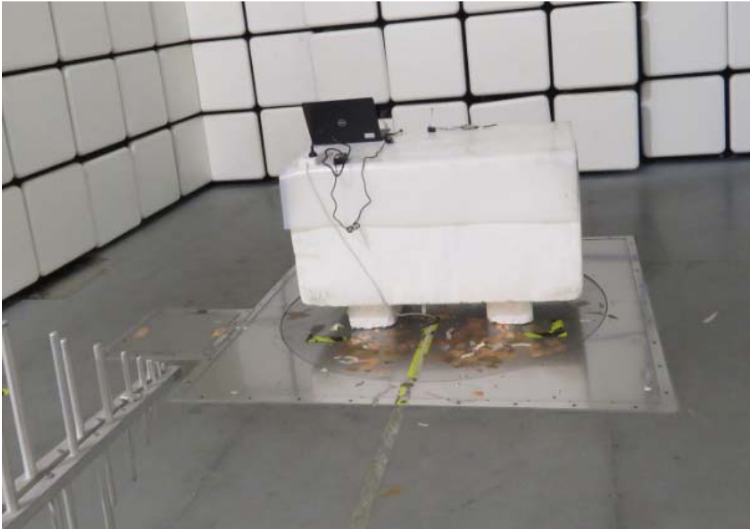
30MHz-1GHz
