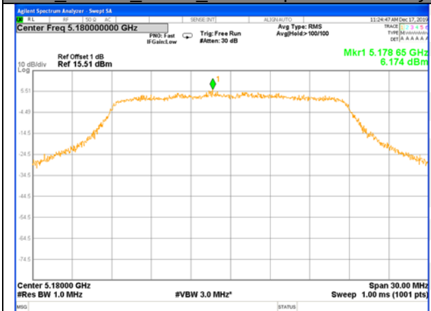
W52_11ac20_Higher_Power Spectrum Density
