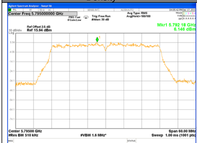
W58_11ac40_Higher_Power Spectrum Density
