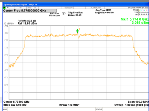
W58_11ac80_Power Density_5775M
