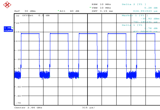
Middle 0.421ms,0.625ms
