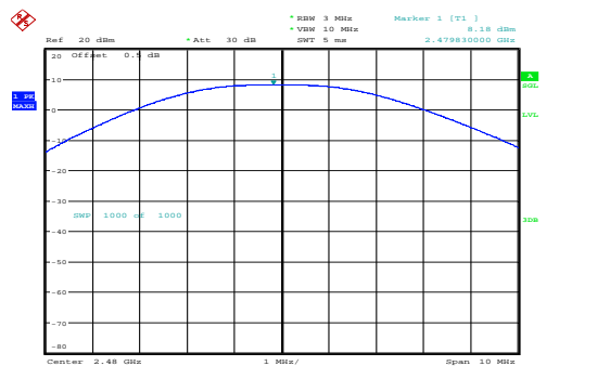
High 8.18dBm
