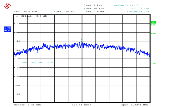
High -11.02dBm/3kHz
