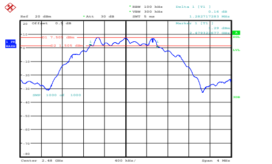
High 1.283MHz
