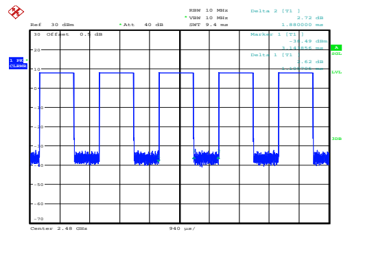
High 1.106ms,1.880ms
