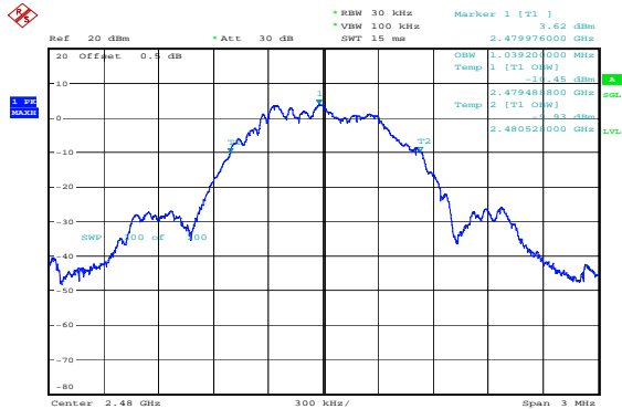
High 1.039MHz
