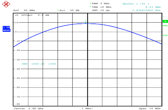
High 8.53dBm
