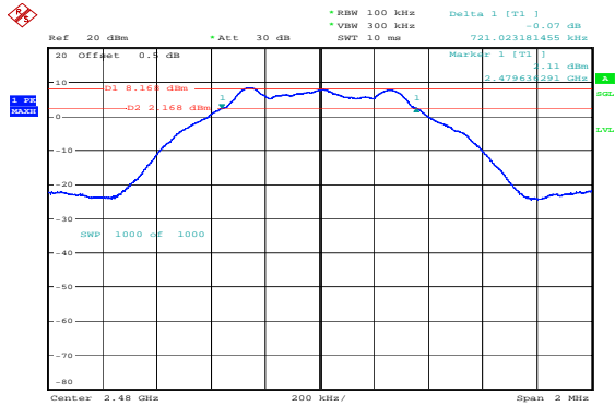
High 0.721MHz
