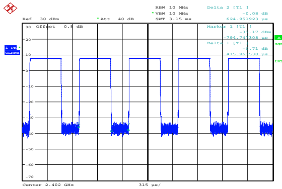
Low 0.416ms,0.625ms
