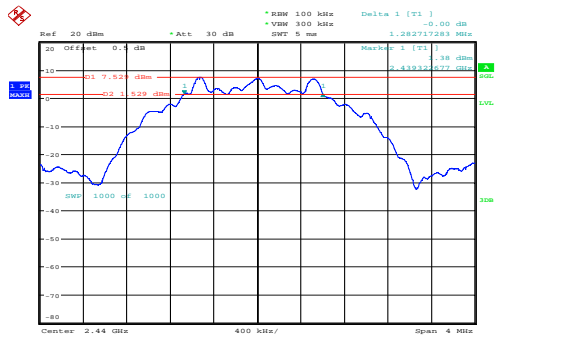
Middle 1.283MHz
