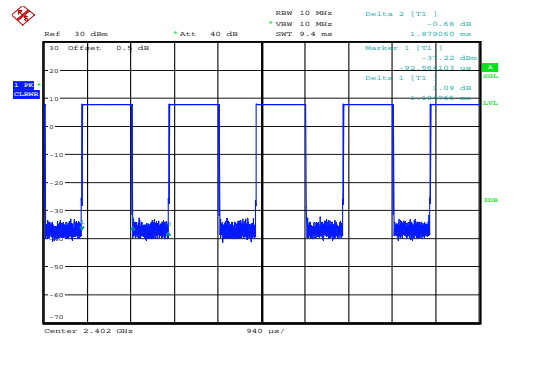
Low 1.105ms,1.879ms
