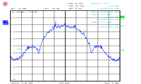
High 2.064MHz
