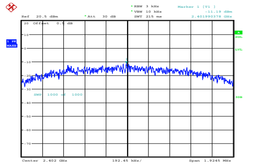
Low -11.19dBm/3kHz
