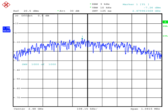
High -7.26dBm/3kHz
