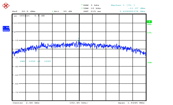
Middle -11.07dBm/3kHz
