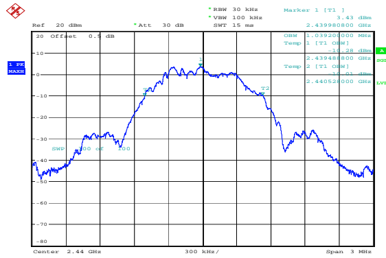
Middle 1.039MHz
