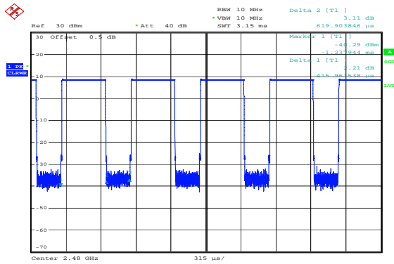
High 0.416ms,0.620ms
