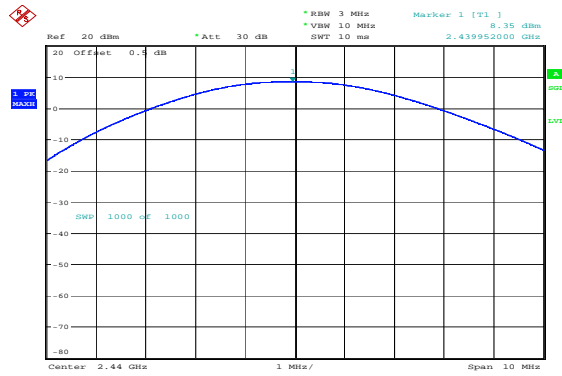
Middle 8.35dBm
