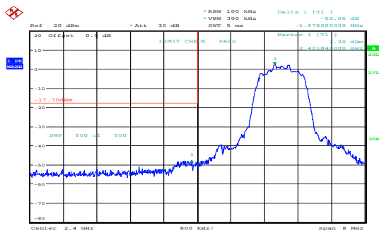
8DPSK_Low 50.06dB
