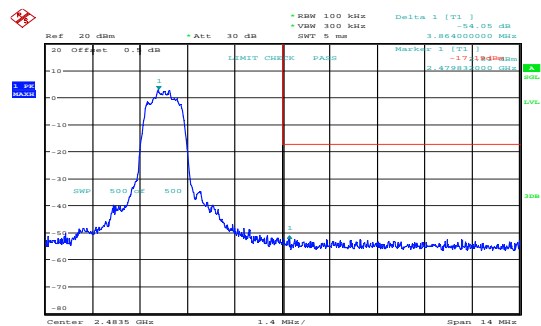
8DPSK_High 54.05dB
