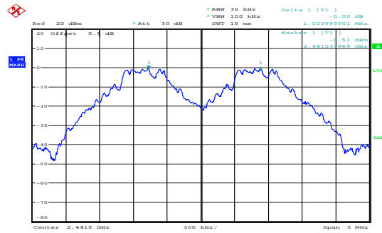
GFSK_Middle 1.001MHz
