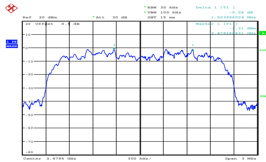
\pi/4 -DQPSK_High 1.004MHz
