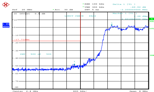
8DPSK_Hopping_Lower 49.92dB
