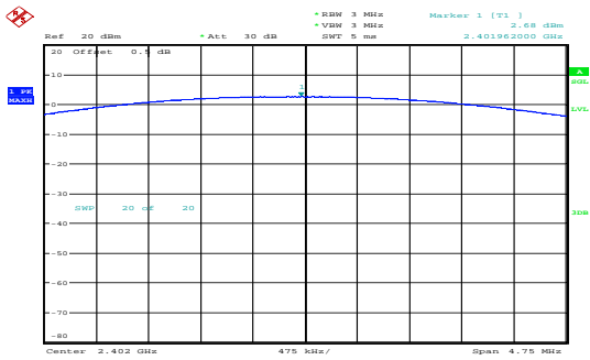
GFSK_Low 2.68dBm
