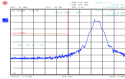
GFSK_Low 50.97dB
