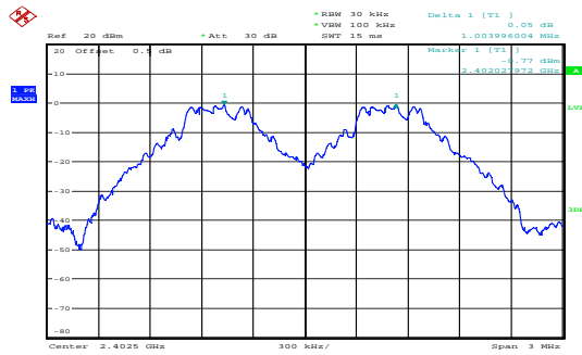
GFSK_Low 1.004MHz
