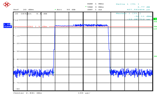
\pi/4 -DQPSK_Hopping_2DH1 0.408ms
