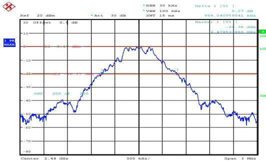
GFSK_High 0.959MHz
