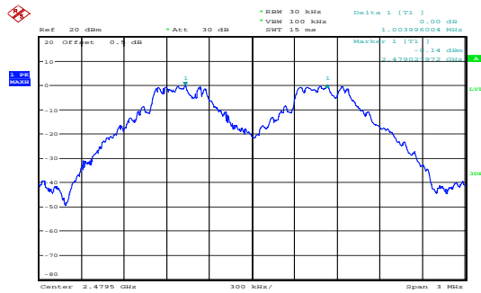
GFSK_High 1.004MHz
