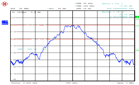
GFSK_Low 0.950MHz
