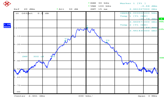
GFSK_Middle 0.864MHz
