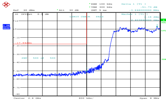
\pi/4 -DQPSK_Hopping_Lower 51.73dB
