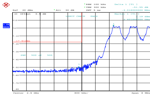
GFSK_Hopping_Lower 51.55dB
