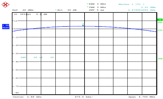
GFSK_High 3.21dBm
