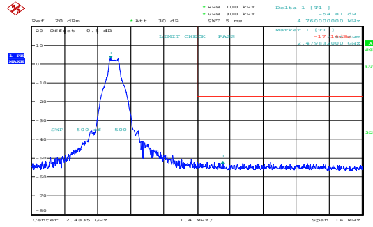
GFSK_High 54.81dB
