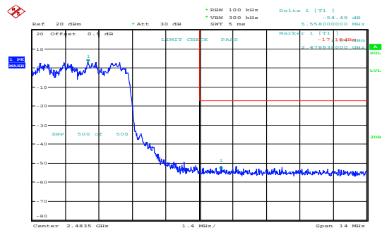
8DPSK_Hopping_Upper 54.48dB
