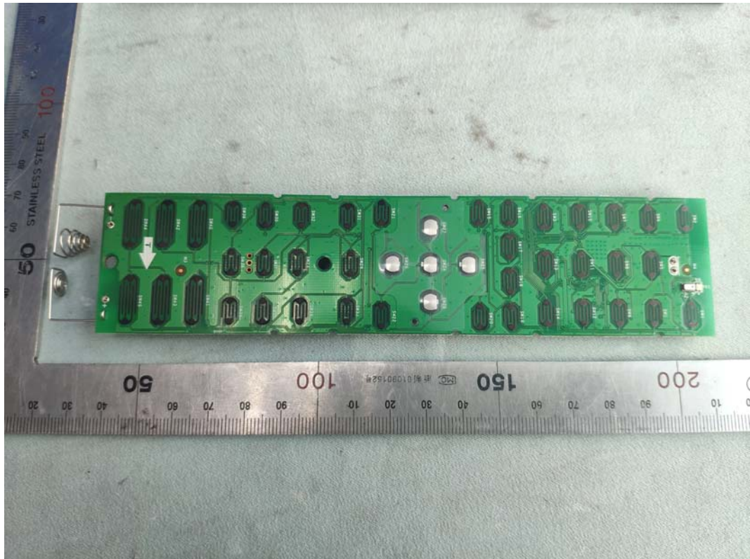
FIGURE 5 REMOTE CONTROL (M/N: ERF3F80H) MAIN BOARD (SOLDERED SIDE)
