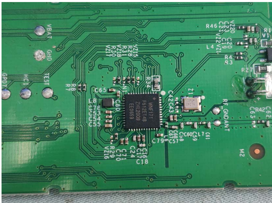
FIGURE 6 REMOTE CONTROL (M/N: ERF3F80H) CHIP & CRYSTAL ON MAIN BOARD
