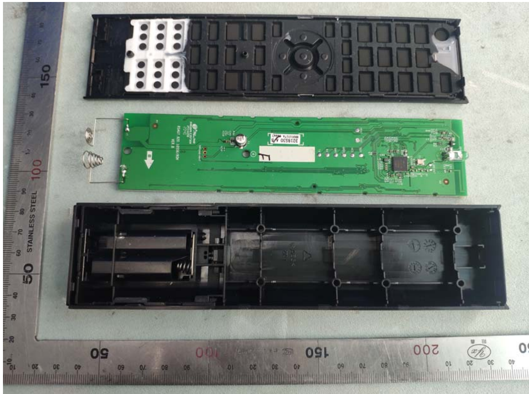
FIGURE 3 REMOTE CONTROL (M/N: ERF3F80H) COVER REMOVED
