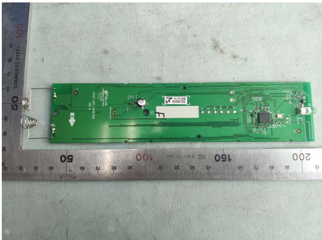
FIGURE 4 REMOTE CONTROL (M/N: ERF3F80H) MAIN BOARD (COMPONENT SIDE)
