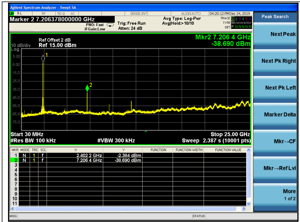
(Channel 0, 30MHz to 25GHz, GFSK)
