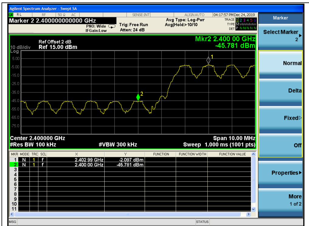
(Channel 0, Band edge with hopping on, GFSK)
