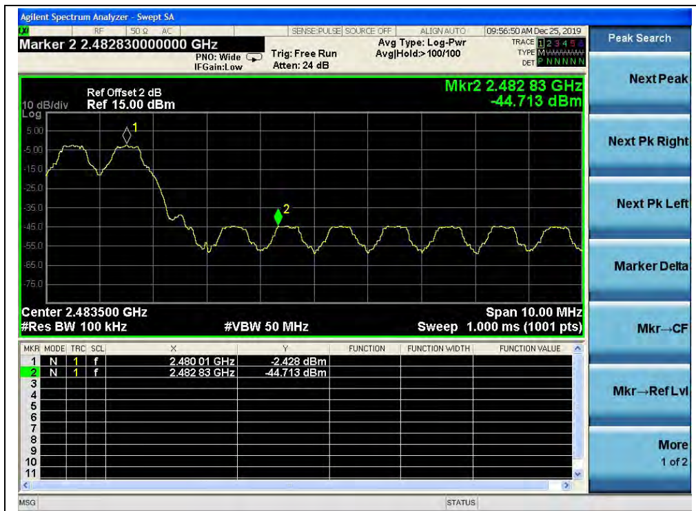
(Channel 78, Band edge with hopping on, GFSK)
