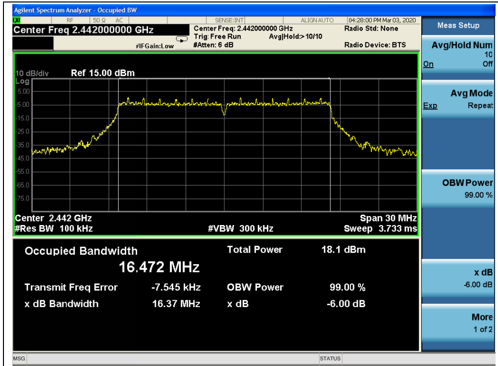
(Channel 7, 802.11g)
