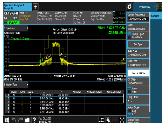
SCC_20M_3569.9MHz_QPSK_FULLRB_CSEpar t96
