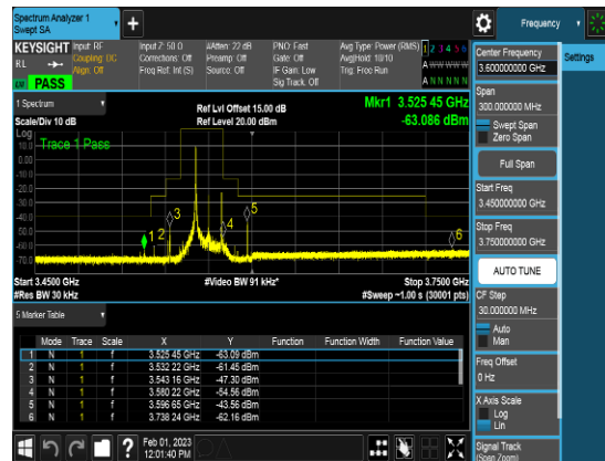
SCC_20M_3569.9MHz_QPSK_1RB_CSEpart96
