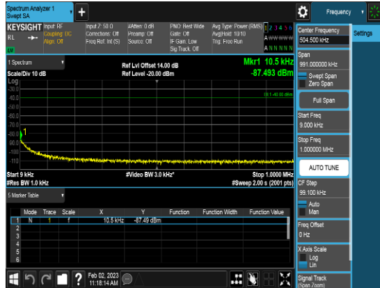
SCC_20M_3630MHz_Q64_FULLLRB_CSE1
