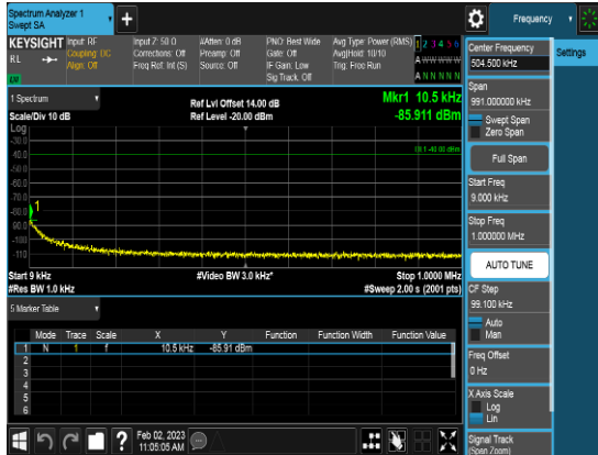
SCC_20M_3569.9MHz_Q16_FULLLRB_CSE1
