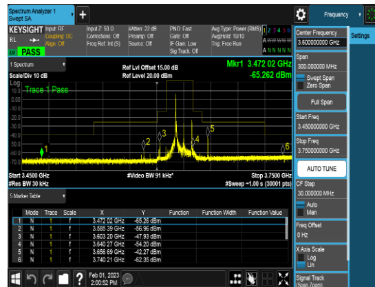
SCC_20M_3630MHz_Q64_1RB_CSEpart96
