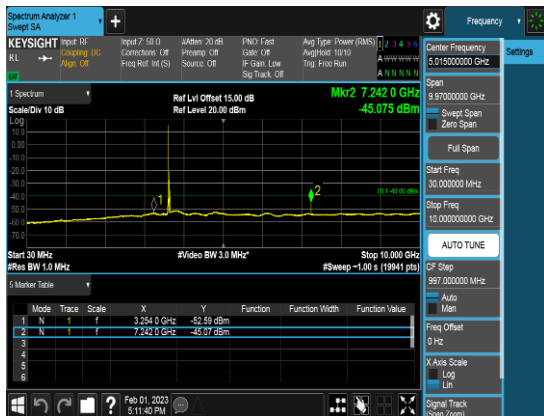
SCC_20M_3630MHz_Q64_1RB_CSE3
