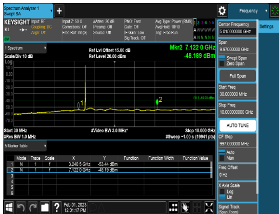
SCC_20M_3569.9MHz_QPSK_1RB_CSE3
