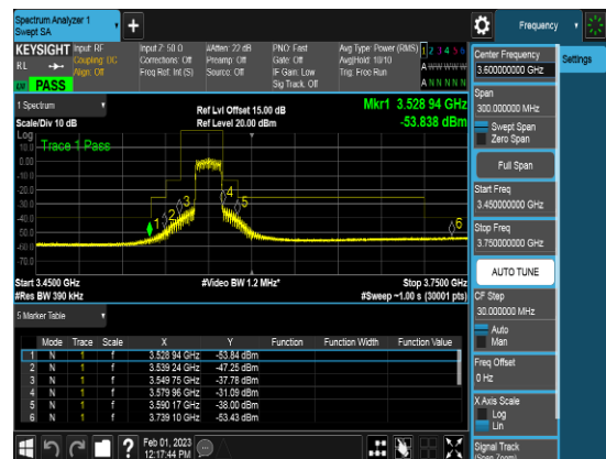
SCC_20M_3569.9MHz_Q64_FULLLRB_CSEpart 6
