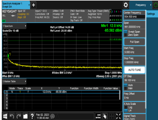
SCC_20M_3569.9MHz_Q64_1RB_CSE1
