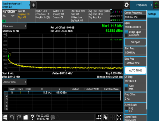
SCC_20M_3630MHz_Q16_1RB_CSE1
