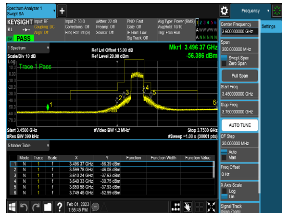
SCC_20M_3630MHz_Q64_FULLLRB_CSEpart96
