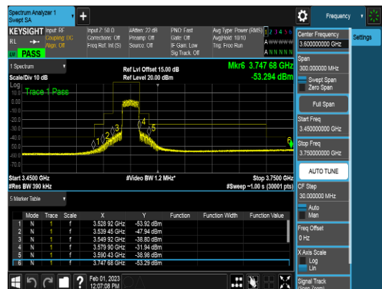
SCC_20M_3569.9MHz_Q16_FULLLRB_CSEpart 6
