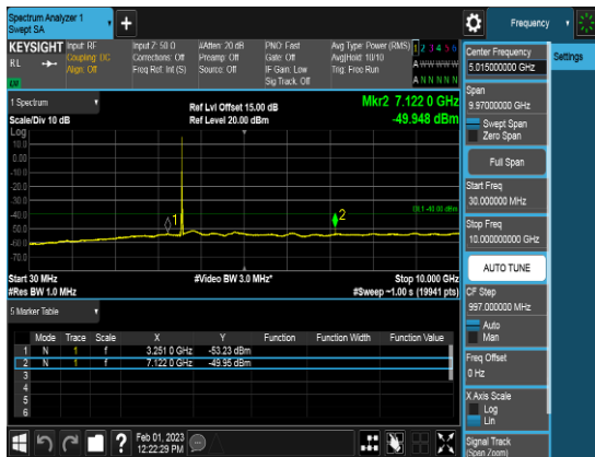
SCC_20M_3569.9MHz_Q64_1RB_CSE3
