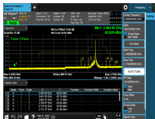
PCC_10M_3675.6MHz_Q64_1RB_CSEpart96
