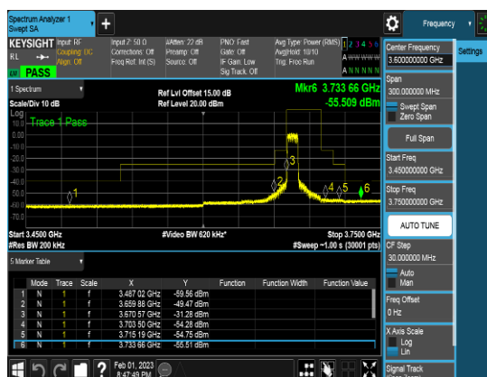
PCC_10M_3675.6MHz_Q16_FULLLRB_CSEpart 6
