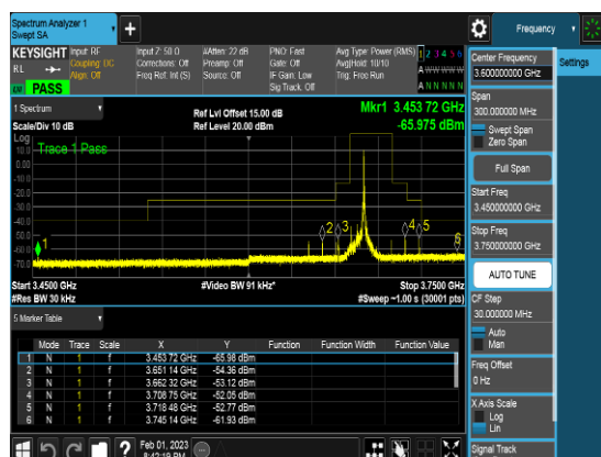
PCC_10M_3675.6MHz_QPSK_1RB_CSEpart96
