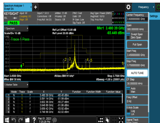
PCC_10M_3615.6MHz_Q64_1RB_CSEpart96
