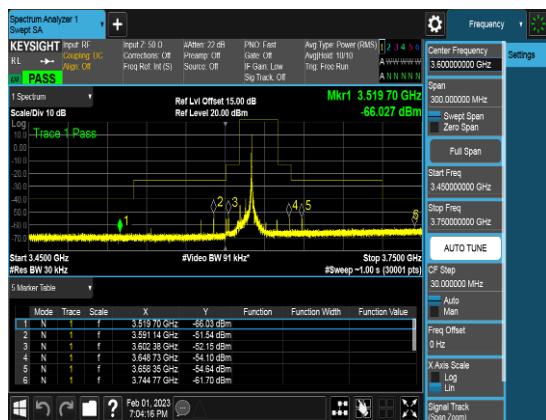
PCC_10M_3615.6MHz_QPSK_1RB_CSEpart96
