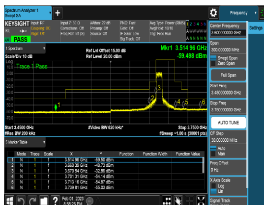
PCC_10M_3675.6MHz_Q64_FULLLRB_CSEpart 6
