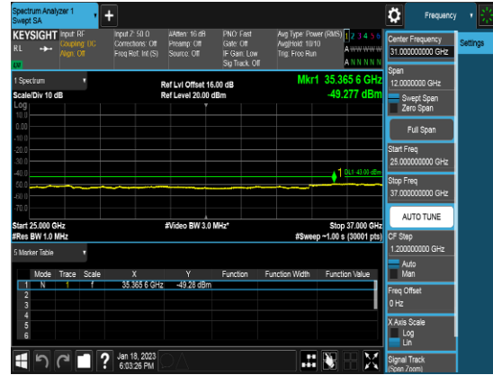
Ant 2_20M_Q64_1RB0_CSEpart96_High channel
