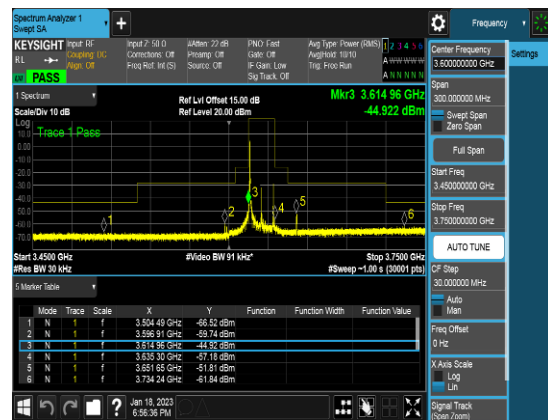
Ant 2_20M_Q16_1RB0_CSEpart96_Middle channel
