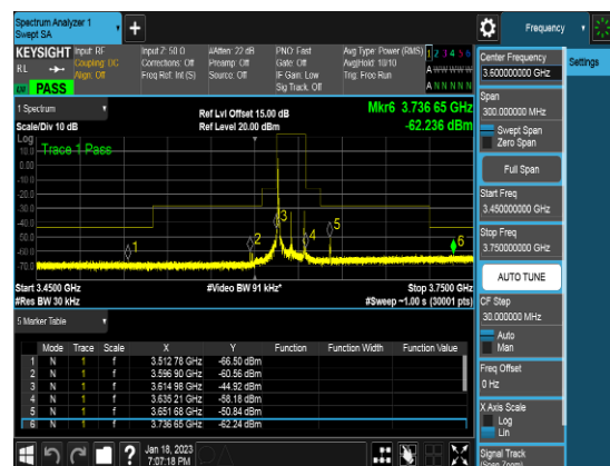
Ant 2_20M_Q64_1RB0_CSEpart96_Middle channel
