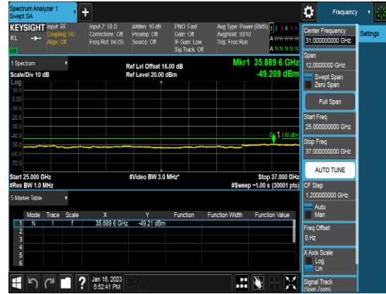
Ant 2_20M_Q16_1RB0_CSEpart96_High channel
