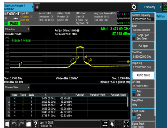
Ant 2_20M_Q16_FULLRB_CSEpart96_Middle channel
