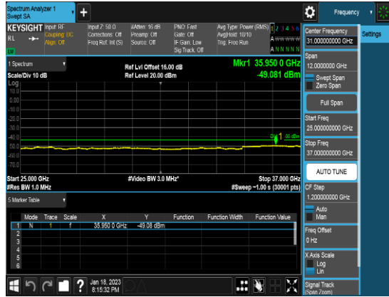
Ant 2_20M_Q64_1RB0_CSE3_Middle channel
