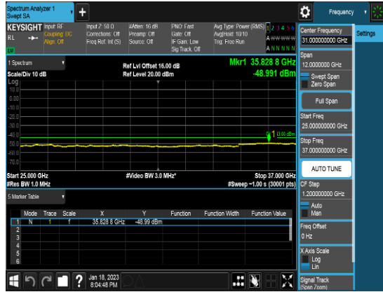
Ant 2_20M_Q16_1RB0_CSE3_Middle channel
