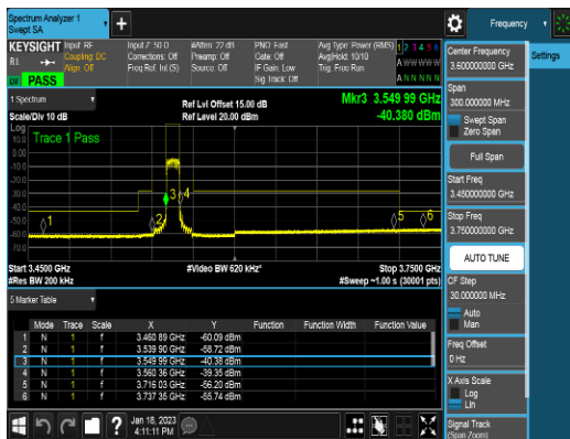
Ant 2_10M_QPSK_FULLLRB_CSEpart96_Low channel
