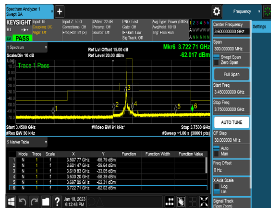
Ant 2_10M_QPSK_1RB0_CSEpart96_Middle channel
