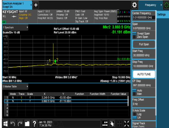
Ant 2_10M_Q64_FULLRB_CSE1_Middle channel
