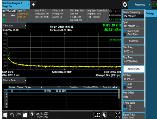
Ant 2_10M_Q64_FULLRB_CSE0a_Middle channel
