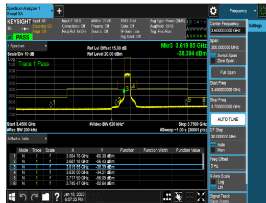
Ant 2_10M_QPSK_FULLLRB_CSEpart96_Middle channel
