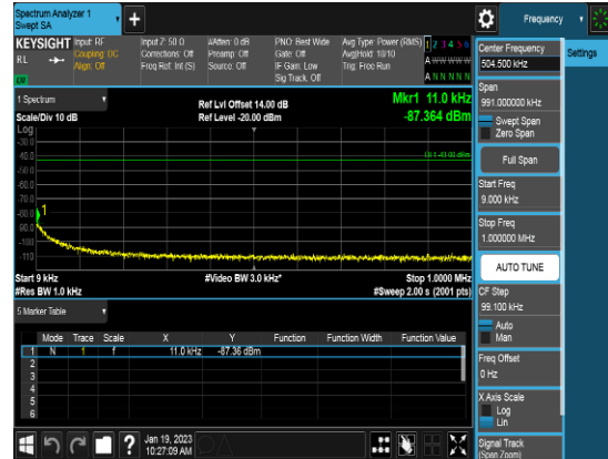
Ant 2_20M_Q16_1RB0_CSE0b_High channel
