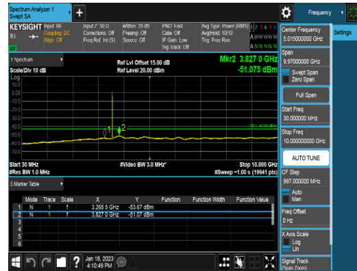
Ant 2_10M_QPSK_FULLLRB_CSE2_High channel
