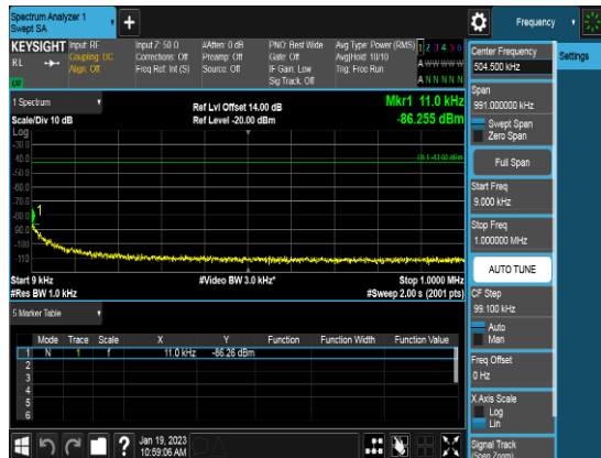
Ant 0_10M_Q16_1RB0_CSE0b_Low channel
