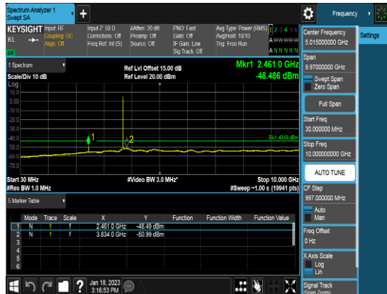
Ant 0_10M_Q16_FULLRB_CSE1_Middle channel
