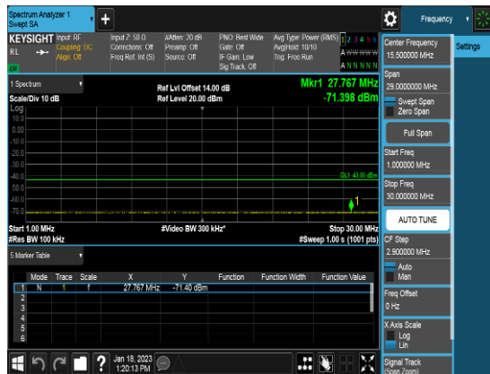
Ant 0_10M_Q64_1RB0_CSE0b_Low channel
