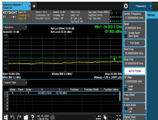
Ant 0_10M_Q16_FULLRB_CSE2_Low channel
