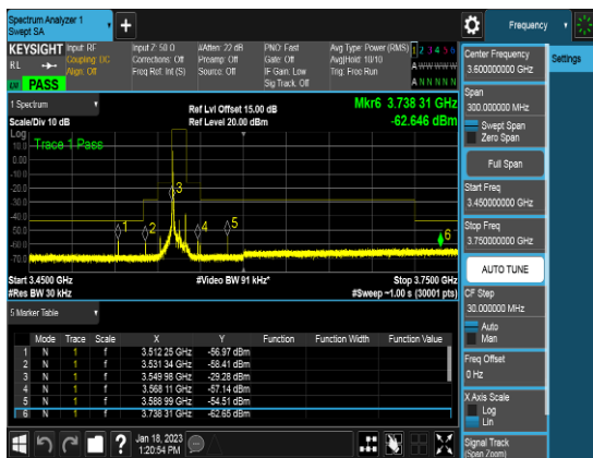
Ant 0_10M_Q64_1RB0_CSEpart96_Low channel
