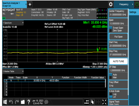
Ant 0_10M_Q16_1RB0_CSE3_Middle channel
