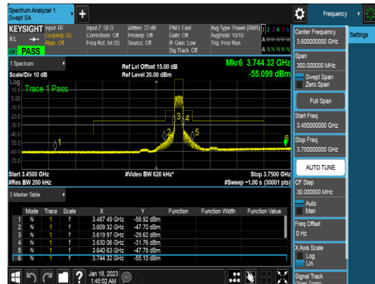
10M_Q64_FULLLRB_CSEpart96_Middle Channel
