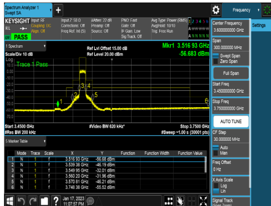
10M_Q64_FULLLRB_CSEpart96_Low channel
