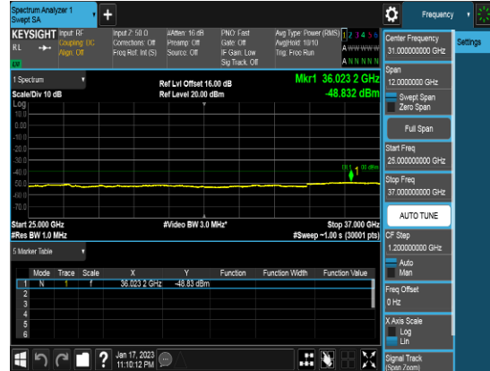
10M_Q64_FULLLRB_CSEpart96_High channel
