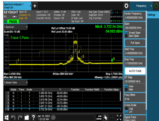
10M_QPSK_FULLLRB_CSEpart96_Middle Channel
