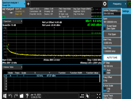
10M_Q64_FULLLRB_CSE0a_Middle Channel
