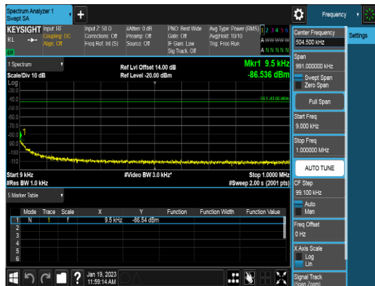
10M_QPSK_FULLLRB_CSE0b_Low channel
