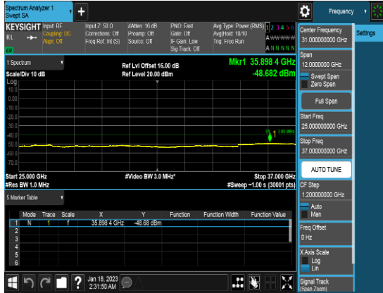
10M_QPSK_FULLLRB_CSE3_Middle Channel
