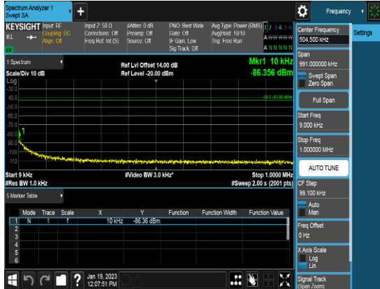
10M_QPSK_1RB0_CSE0a_Middle Channel
