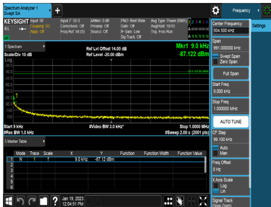
20M_Q16_1RB0_CSE0b_Low channel
