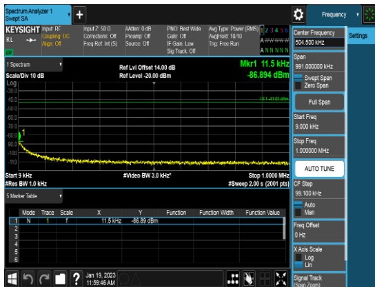
10M_QPSK_1RB0_CSE0b_Middle Channel
