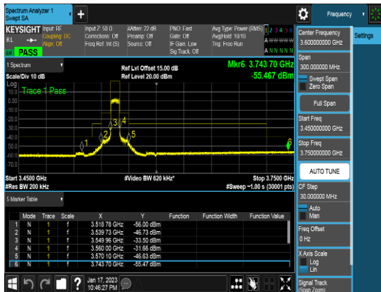
10M_QPSK_FULLLRB_CSEpart96_Low channel
