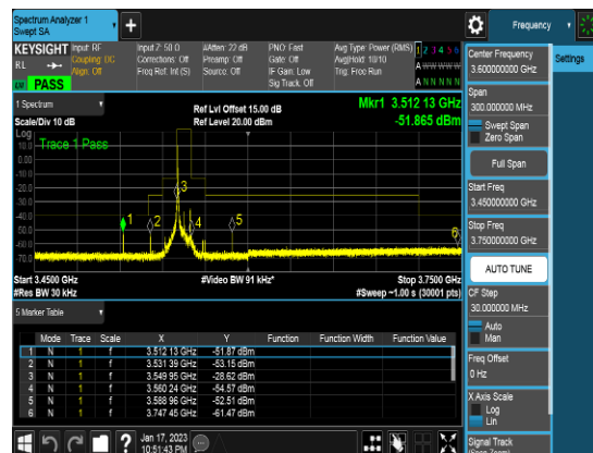
10M_QPSK_1RB_CSE0b_High channel
