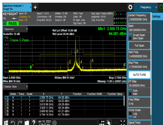
10M_QPSK_1RB0_CSEpart96_Middle Channel
