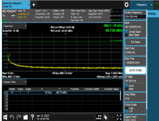
20M_Q16_1RB0_CSE0a_Middle Channel
