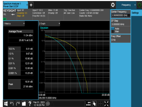
SCC_20M_3569.9MHz_QPSK_FULLRB_PAPR
