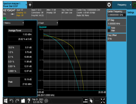
SCC_20M_3690MHz_Q64_FULLRB_PAPR
