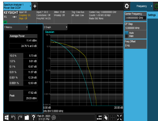
SCC_20M_3690MHz_QPSK_FULLRB_PAPR
