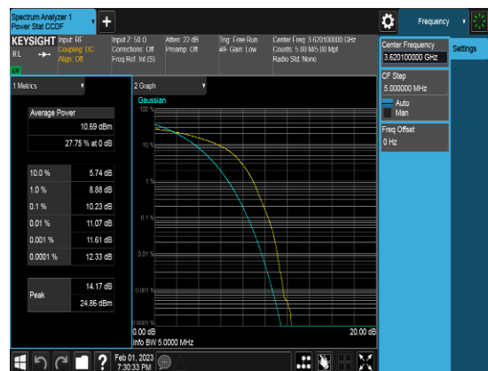
PCC_20M_3620.1MHz_QPSK_FULLRB_PAPR
