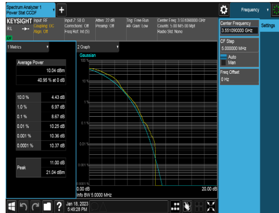
Ant 2_20M_Q16_FULLRB_PAPR_High channel
