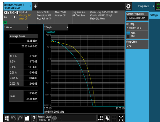
PCC_10M_3675.6MHz_QPSK_FULLRB_PAPR
