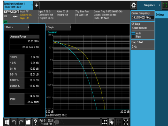
PCC_20M_3620.1MHz_Q64_FULLRB_PAPR
