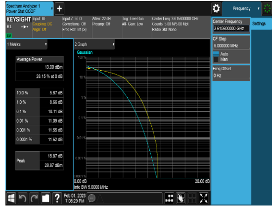
PCC_10M_3615.6MHz_Q64_FULLRB_PAPR
