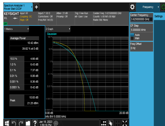
Ant 0_10M_QPSK_FULLLRB_PAPR_Middle channel
