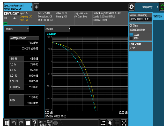
Ant 0_20M_Q64_FULLLRB_PAPR_Middle channel
