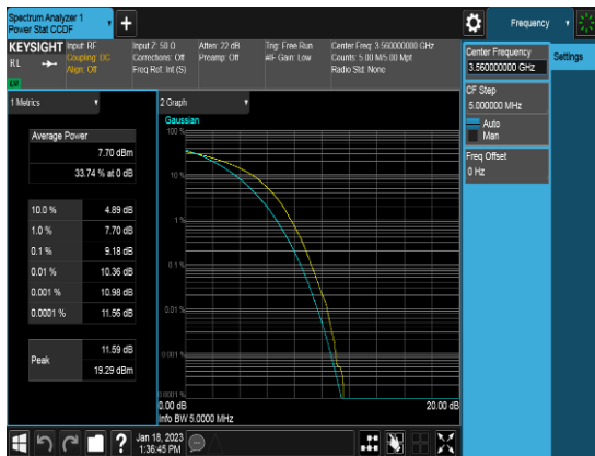
Ant 0_20M_Q16_FULLLRB_PAPR_Low channel
