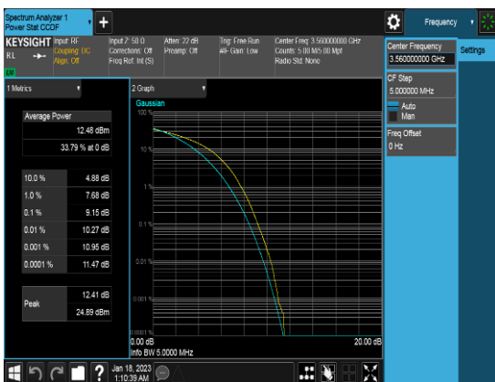
20M_Q64_FULLLRB_PAPR_Low channel
