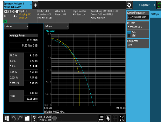
20M_QPSK_FULLRB_PAPR_High channel
