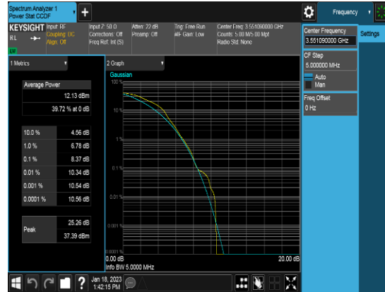
Ant 0_20M_Q16_FULLLRB_PAPR_High channel
