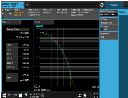
Ant 0_10M_Q16_FULLRB_PAPR_Low channel
