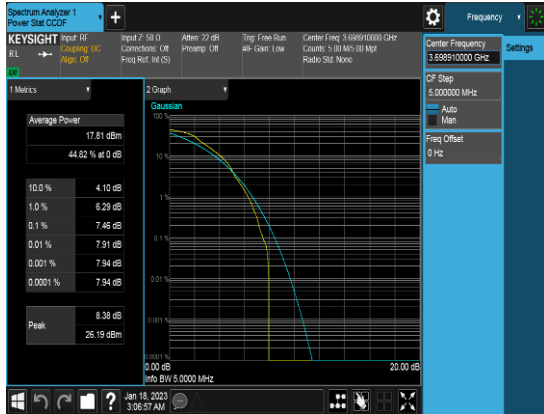
20M_QPSK_1RB0_PAPR_Middle channel
