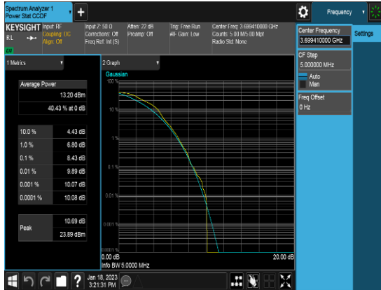
Ant 0_10M_Q16_1RB0_PAPR_Middle channel
