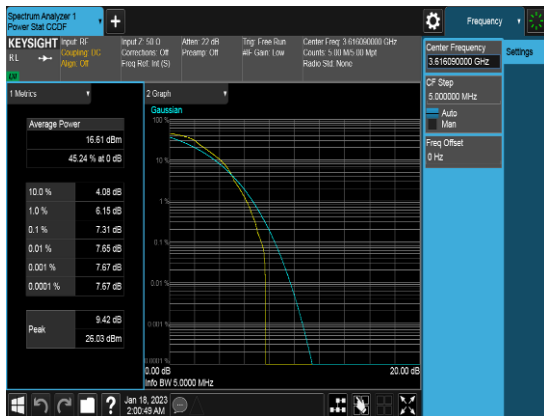
20M_QPSK_FULLRB_PAPR_Low channel
