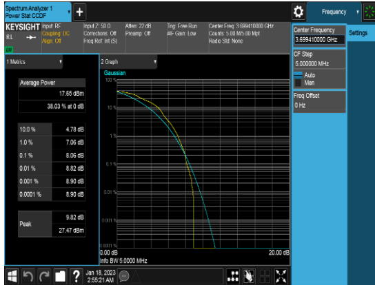
10M_Q64_1RB0_PAPR_Middle channel
