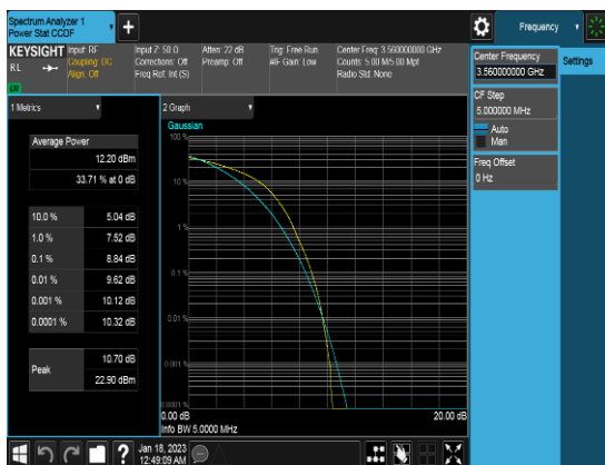
20M_QPSK_FULLRB_PAPR_Low channel
