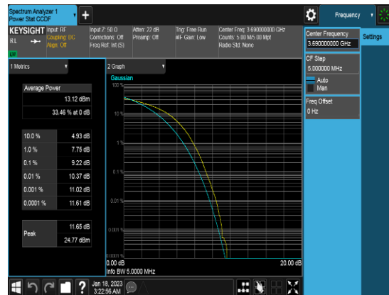
20M_Q64_FULLLRB_PAPR_Middle channel
