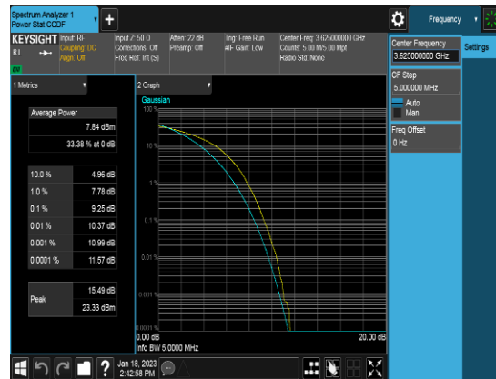
Ant 0_20M_Q16_FULLLRB_PAPR_Middle channel
