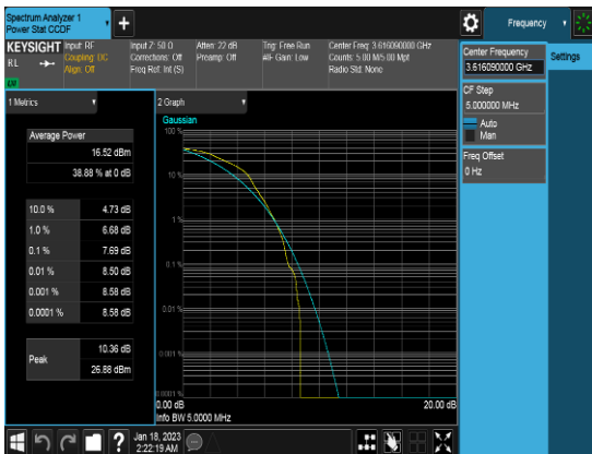
20M_Q64_FULLLRB_PAPR_Low channel
