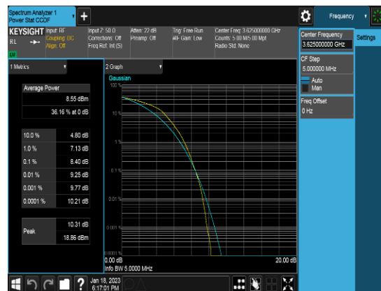
Ant 2_10M_Q16_FULLLRB_PAPR_Middle channel
