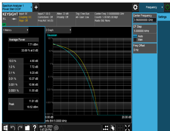
Ant 0_20M_Q64_FULLLRB_PAPR_Low channel
