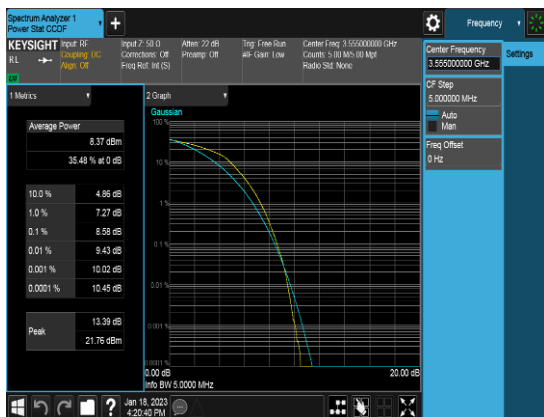
Ant 2_10M_Q16_FULLLRB_PAPR_Low channel
