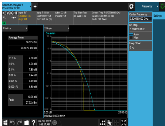
10M_Q64_FULLRB_PAPR_Low channel
