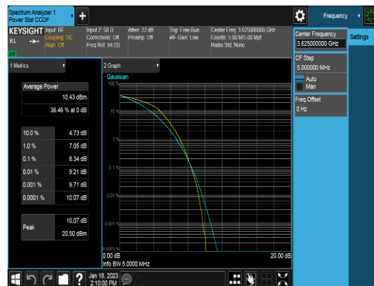
Ant 0_10M_Q16_FULLRB_PAPR_Middle channel
