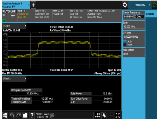
SCC_20M_3634.9MHz_QPSK_FULLLRB_OBW
