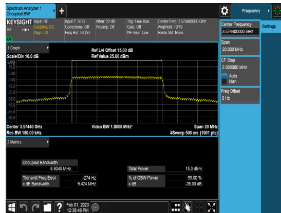
SCC_10M_3574.4MHz_QPSK_FULLLRB_OBW
