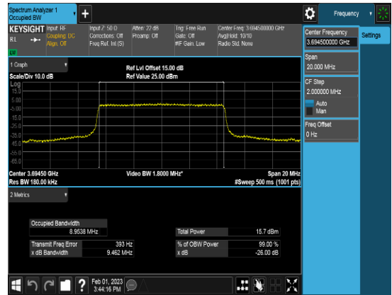
SCC_10M_3694.5MHz_QPSK_FULLLRB_OBW
