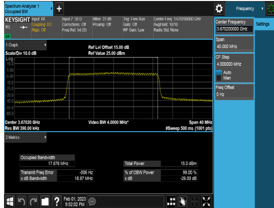
PCC_20M_3670.2MHz_QPSK_FULLLRB_OBW
