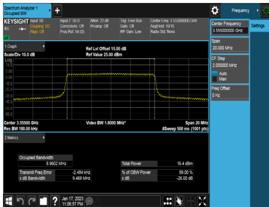
10M_Q64_FULLLRB_OBW_Low channel
