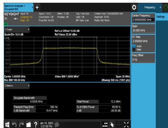
Ant 0_10M_Q64_FULLLRB_OBW_Middle channel
