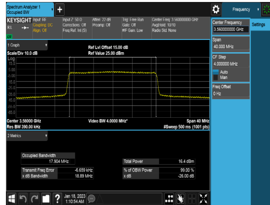
20M_QPSK_FULLLRB_OBW_High channel
