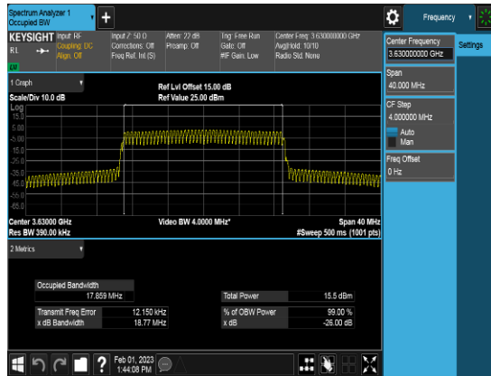
SCC_20M_3630MHz_QPSK_FULLLRB_OBW
