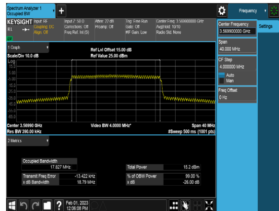
SCC_20M_3569.9MHz_QPSK_FULLLRB_OBW
