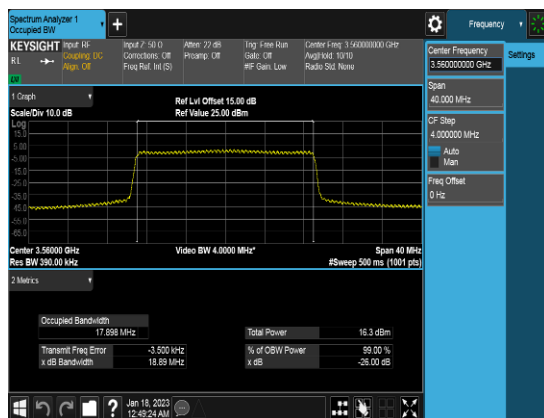
20M_QPSK_FULLLRB_OBW_Low channel
