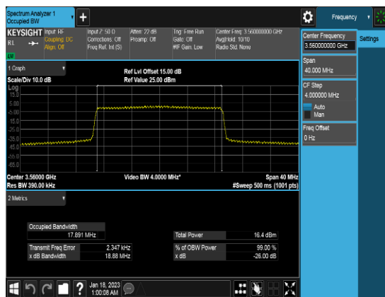
20M_Q16_FULLLRB_OBW_Low channel
