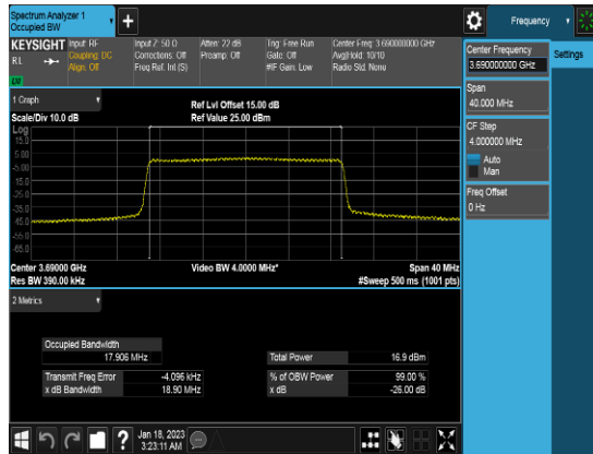
20M_Q64_FULLLRB_OBW_Middle channel
