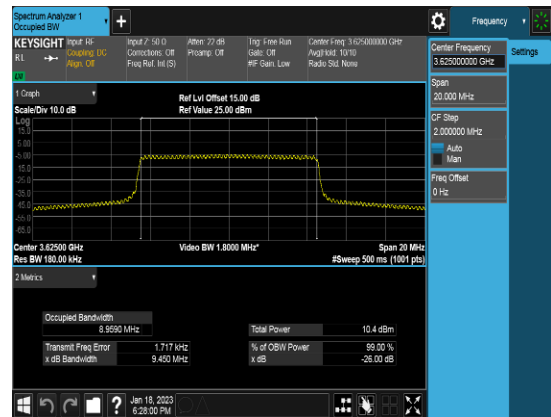
Ant 2_10M_Q64_FULLLRB_OBW_Middle channel
