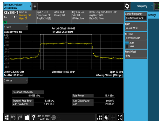
10M_Q64_FULLLRB_OBW_Middle channel
