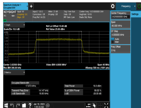
20M_QPSK_FULLLRB_OBW_Middle channel
