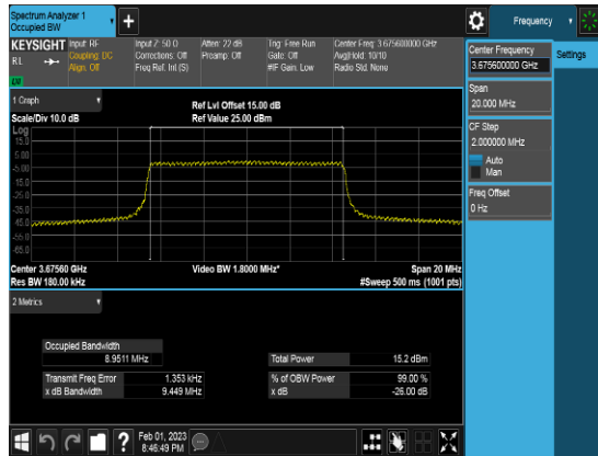
PCC_10M_3675.6MHz_QPSK_FULLLRB_OBW
