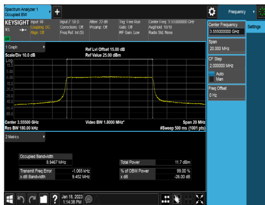
Ant 0_10M_Q64_FULLLRB_OBW_Low channel
