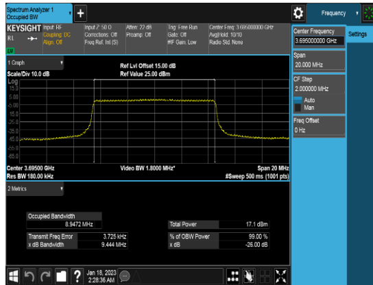
10M_QPSK_FULLLRB_OBW_Middle channel
