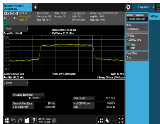
20M_Q16_FULLLRB_OBW_Middle channel
