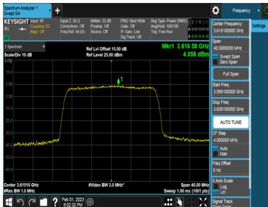
PCC_20M_3615.1MHz_QPSK_FULLRB_PSD
