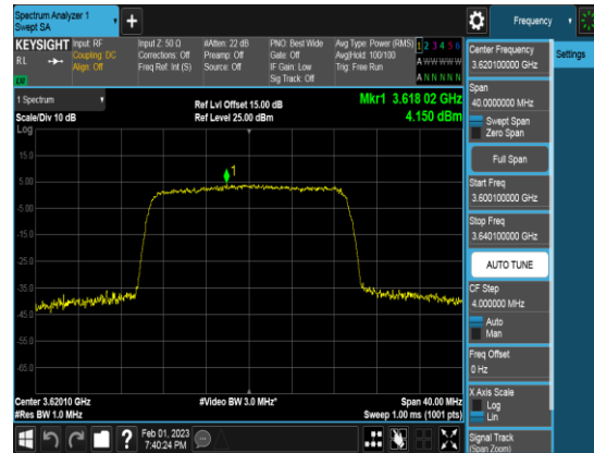
PCC_20M_3620.1MHz_Q64_FULLLRB_PSD
