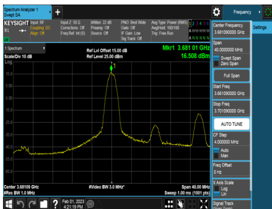
SCC_20M_3690MHz_QPSK_1RB0_PSD
