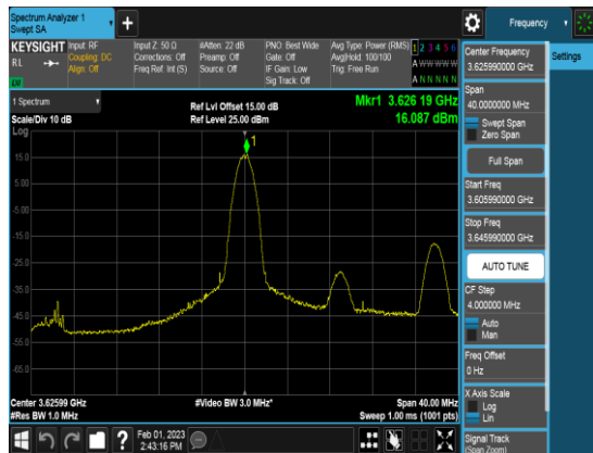
SCC_20M_3634.9MHz_QPSK_1RB0_PSD
