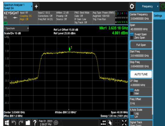
SCC_20M_3634.9MHz_QPSK_FULLRB_PSD
