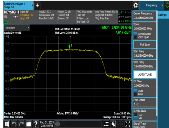
SCC_10M_3634.5MHz_Q64_FULLRB_PSD
