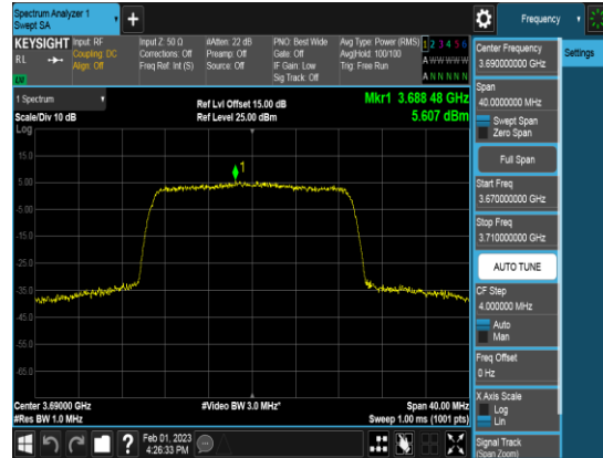
SCC_20M_3690MHz_Q64_FULLLRB_PSD
