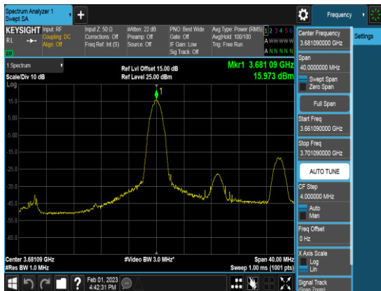
SCC_20M_3690MHz_QPSK_1RB0_PSD
