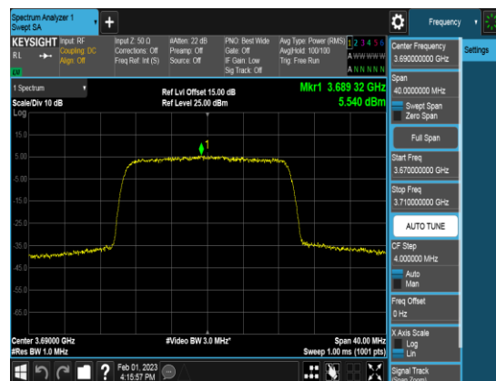
SCC_20M_3690MHz_QPSK_FULLLRB_PSD
