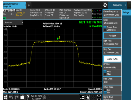
SCC_20M_3690MHz_QPSK_FULLLRB_PSD
