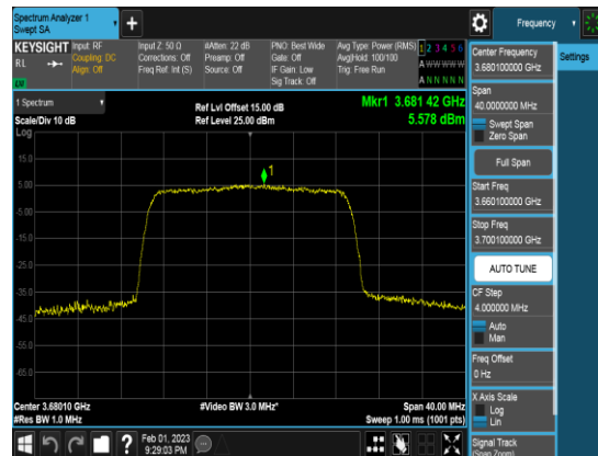
PCC_20M_3680.1MHz_QPSK_FULLLRB_PSD
