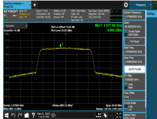
SCC_20M_3579.8MHz_Q64_FULLLRB_PSD
