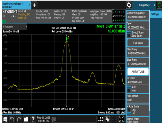
SCC_20M_3690MHz_Q64_1RB0_PSD
