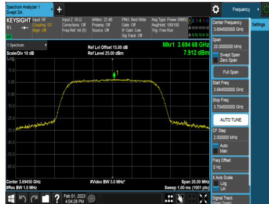
SCC_10M_3694.5MHz_QPSK_FULLLRB_PSD
