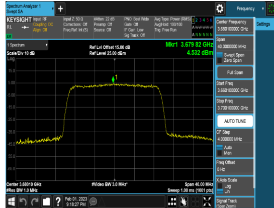
PCC_20M_3680.1MHz_Q64_FULLLRB_PSD
