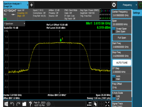
PCC_10M_3615.6MHz_QPSK_FULLRB_PSD
