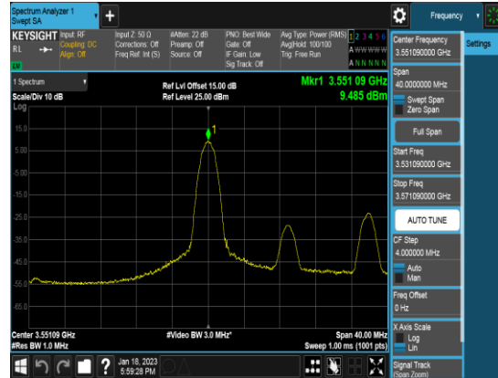
Ant 2_20M_Q64_FULLLRB_PSD_High channel
