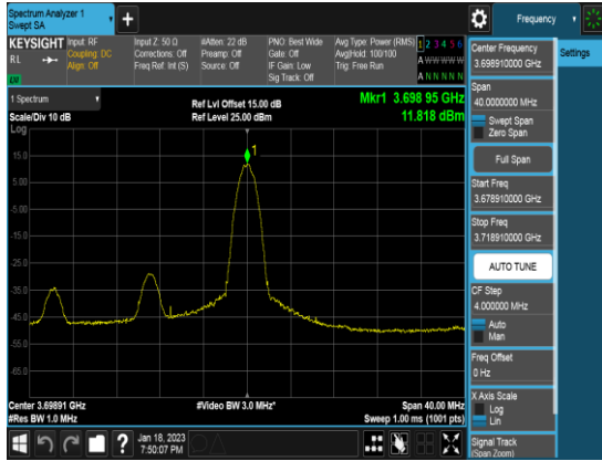
Ant 2_20M_QPSK_1RB0_PSD_Middle channel
