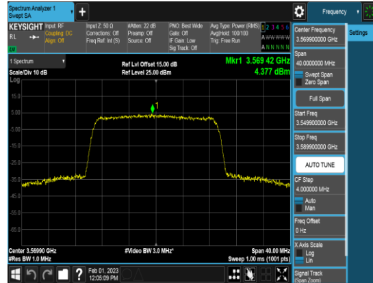
SCC_20M_3569.9MHz_Q64_FULLRB_PSD
