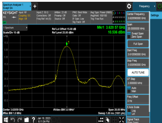
Ant 2_10M_QPSK_FULLRB_PSD_Low channel
