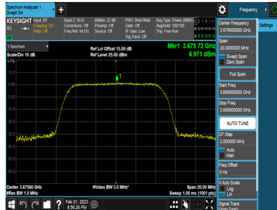
PCC_10M_3675.6MHz_QPSK_FULLRB_PSD
