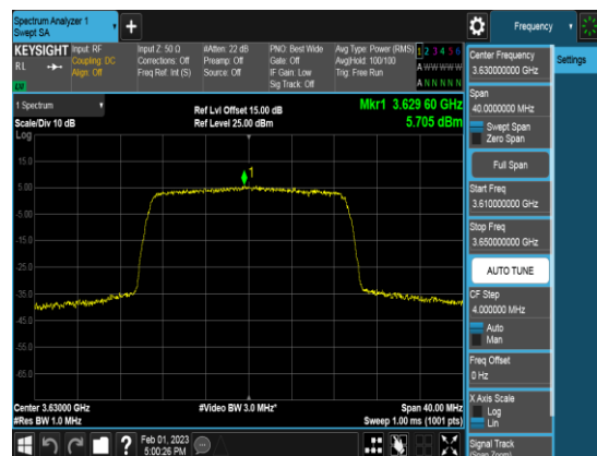
SCC_20M_3630MHz_QPSK_FULLLRB_PSD
