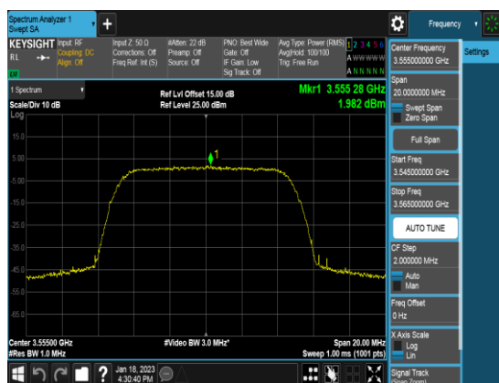
Ant 2_10M_Q64_FULLLRB_PSD_Low channel
