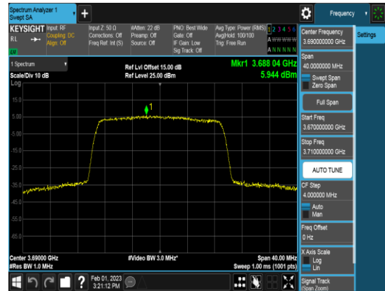
SCC_20M_3690MHz_Q64_FULLRB_PSD
