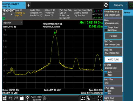
SCC_20M_3630MHz_QPSK_1RB0_PSD
