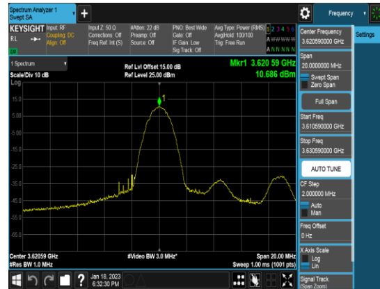
Ant 2_10M_Q64_FULLLRB_PSD_High channel
