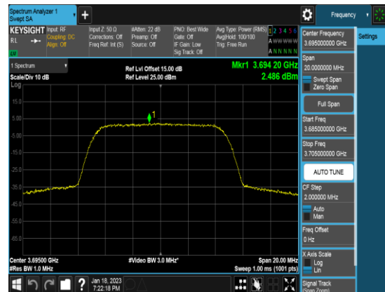
Ant 2_10M_Q16_FULLRB_PSD_Middle channel
