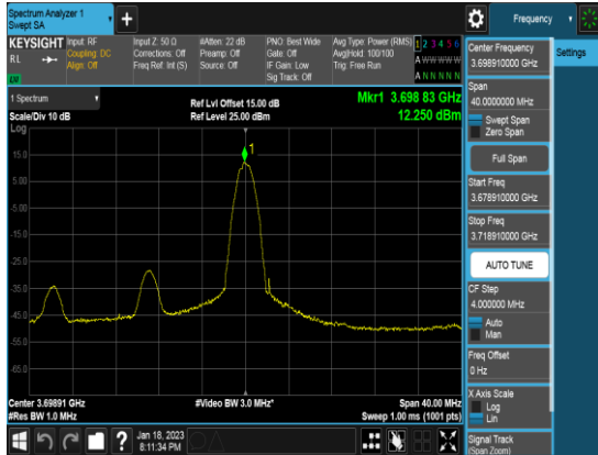
Ant 2_20M_Q64_1RB0_PSD_Middle channel
