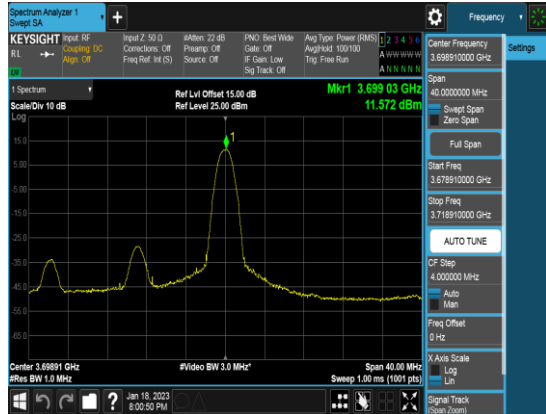
Ant 2_20M_Q16_1RB0_PSD_Middle channel
