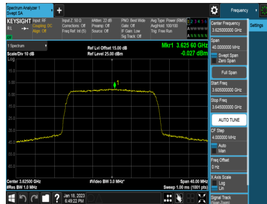
Ant 2_20M_Q16_FULLLRB_PSD_Middle channel
