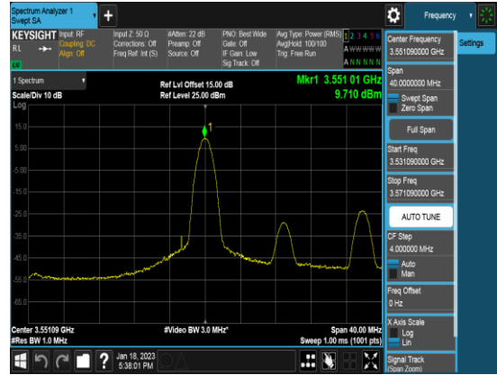
Ant 2_20M_QPSK_FULLRB_PSD_High channel
