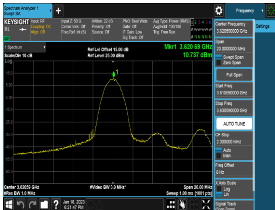
Ant 2_10M_Q16_FULLRB_PSD_Low channel
