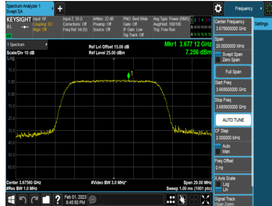
PCC_10M_3675.6MHz_Q64_FULLRB_PSD
