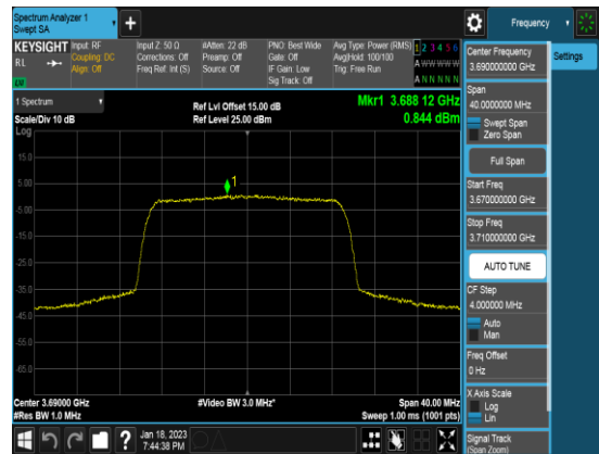
Ant 2_20M_QPSK_FULLRB_PSD_Middle channel
