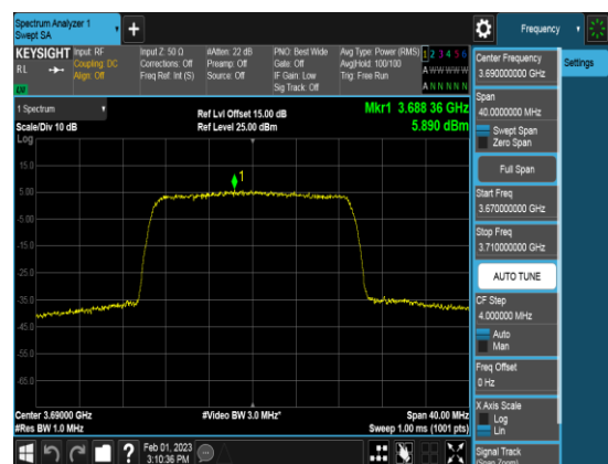
SCC_20M_3690MHz_QPSK_FULLRB_PSD
