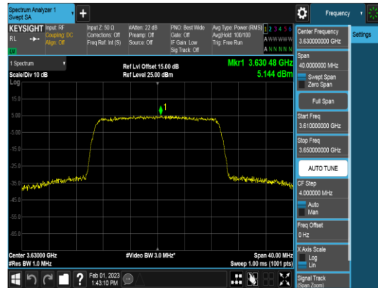
SCC_20M_3630MHz_Q64_FULLLRB_PSD
