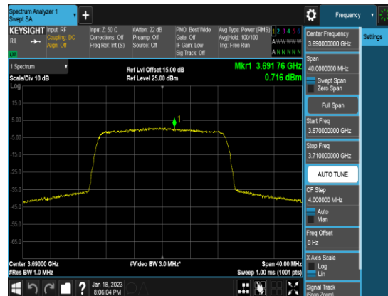
Ant 2_20M_Q64_FULLLRB_PSD_Middle channel
