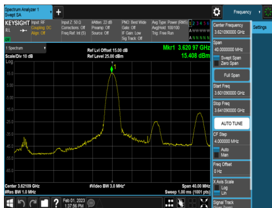
SCC_20M_3630MHz_QPSK_1RB0_PSD
