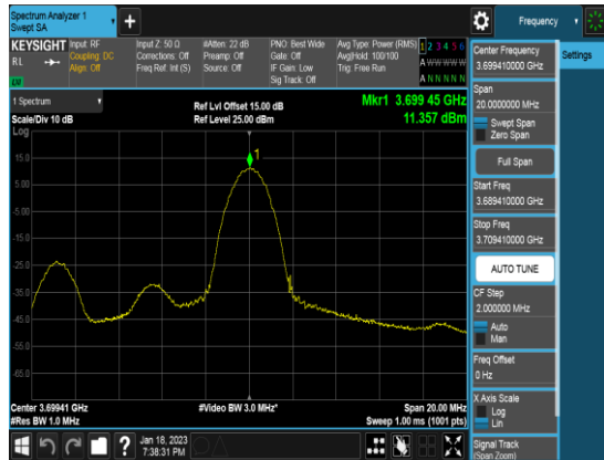
Ant 2_10M_Q64_1RB0_PSD_Low channel
