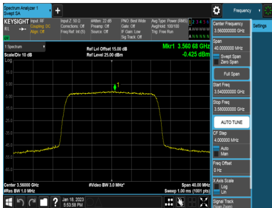
Ant 2_20M_Q64_FULLLRB_PSD_Low channel
