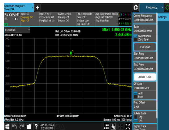
Ant 2_10M_Q64_FULLLRB_PSD_Middle channel
