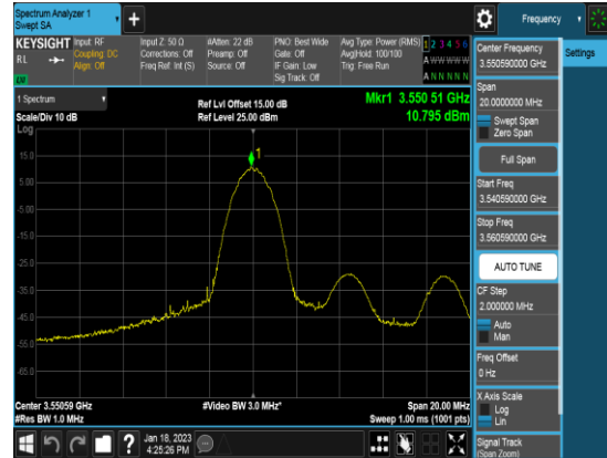
Ant 2_10M_Q16_FULLRB_PSD_High channel
