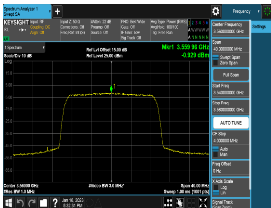
Ant 2_20M_QPSK_FULLRB_PSD_Low channel
