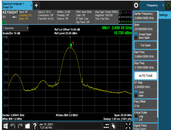
Ant 2_10M_Q16_1RB0_PSD_Middle channel
