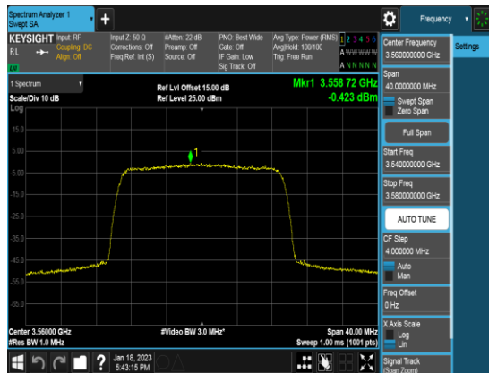
Ant 2_20M_Q16_FULLLRB_PSD_Low channel
