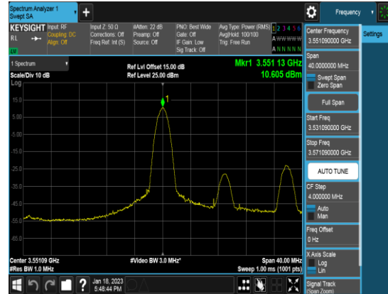
Ant 2_20M_Q16_FULLLRB_PSD_High channel
