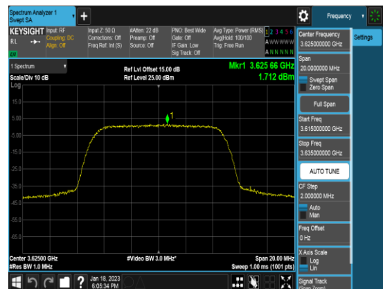
Ant 2_10M_QPSK_FULLRB_PSD_Middle channel
