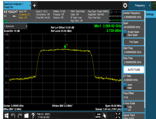
SCC_20M_3569.9MHz_QPSK_FULLRB_PSD
