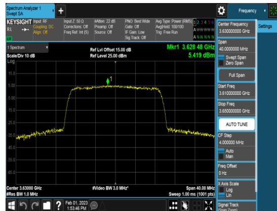
SCC_20M_3630MHz_QPSK_FULLLRB_PSD
