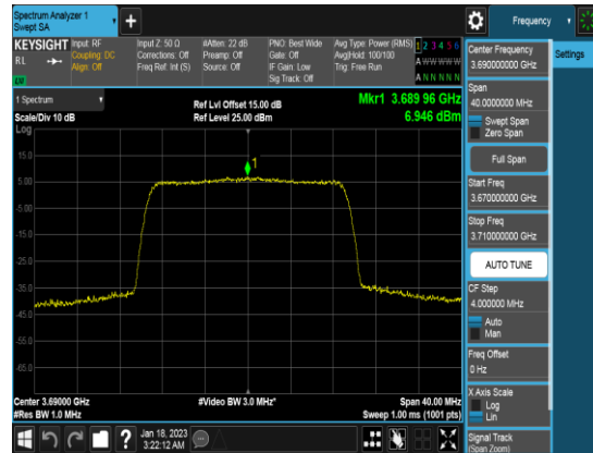
20M_Q64_FULLLRB_PSD_Middle channel
