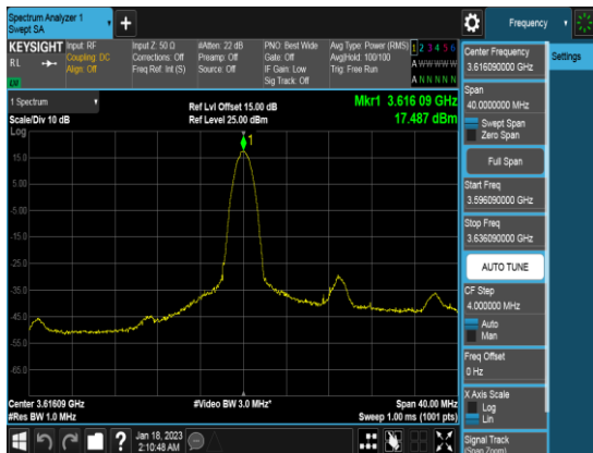
20M_Q16_FULLRB_PSD_Low channel
