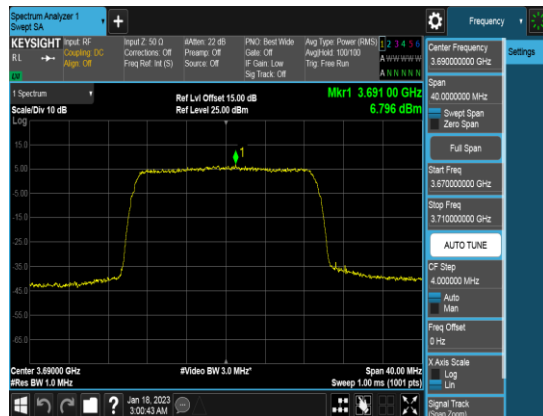
20M_QPSK_FULLRB_PSD_Middle channel
