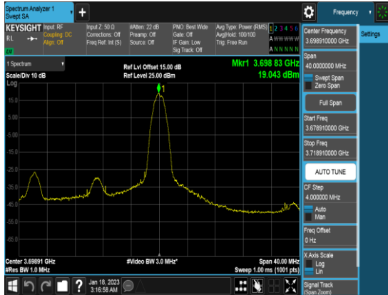
20M_Q16_1RB0_PSD_Middle channel
