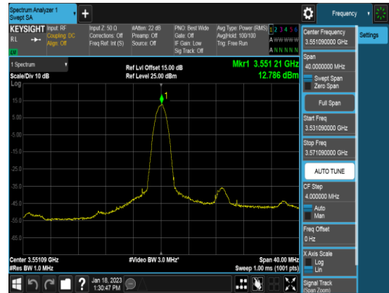
Ant 0_20M_QPSK_FULLRB_PSD_High channel
