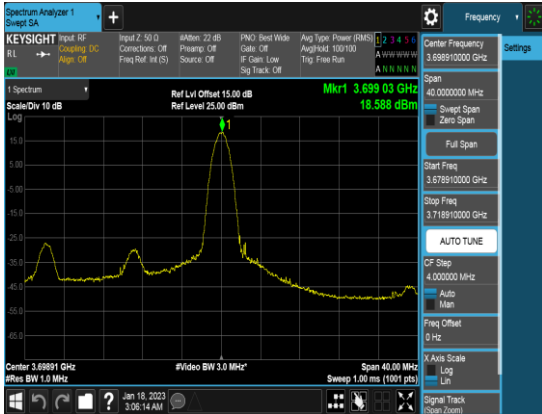
20M_QPSK_1RB0_PSD_Middle channel
