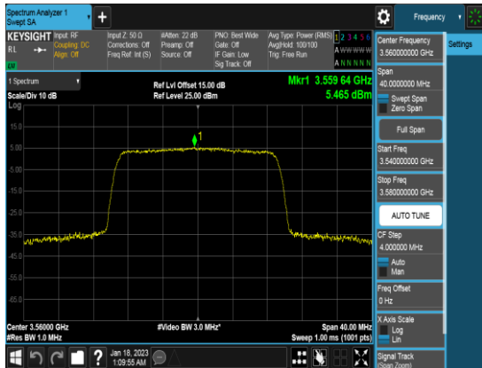
20M_Q64_FULLLRB_PSD_Low channel
