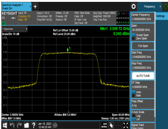
20M_QPSK_FULLRB_PSD_Low channel
