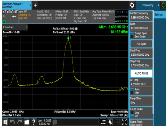
20M_Q64_1RB0_PSD_Middle channel
