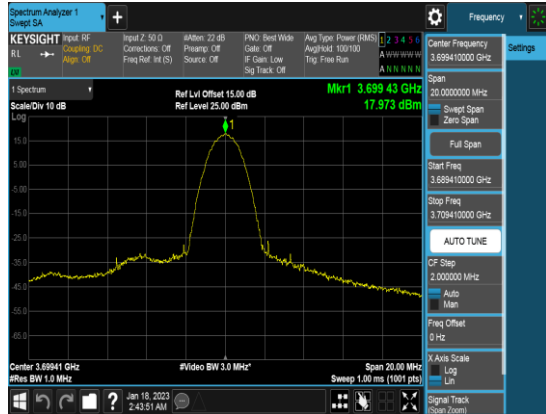
10M_Q16_1RB0_PSD_Middle channel
