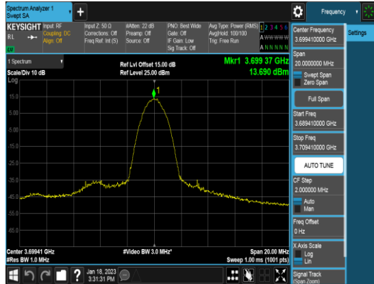
Ant 0_10M_Q64_1RB0_PSD_Middle channel
