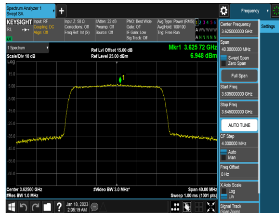
20M_Q16_FULLRB_PSD_Middle channel
