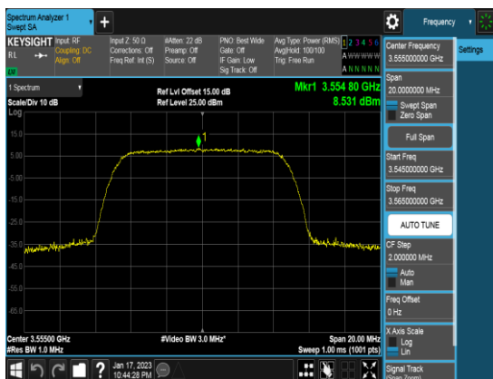
10M_QPSK_FULLRB_PSD_Low channe
