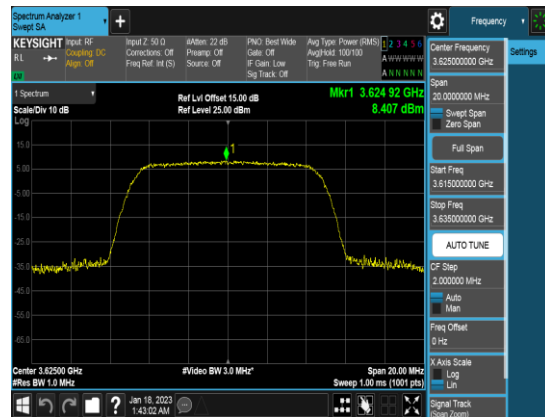
10M_Q64_FULLRB_PSD_Middle channel
