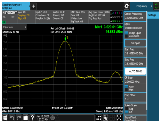
10M_QPSK_FULLRB_PSD_Low channe
