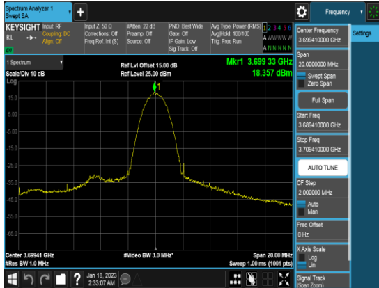
10M_QPSK_1RB0_PSD_Middle channelD
