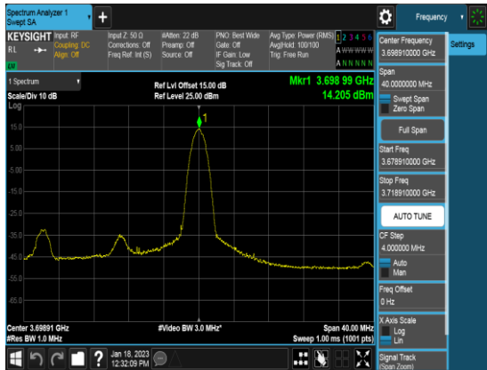
Ant 0_20M_Q16_1RB0_PSD_Middle channel
