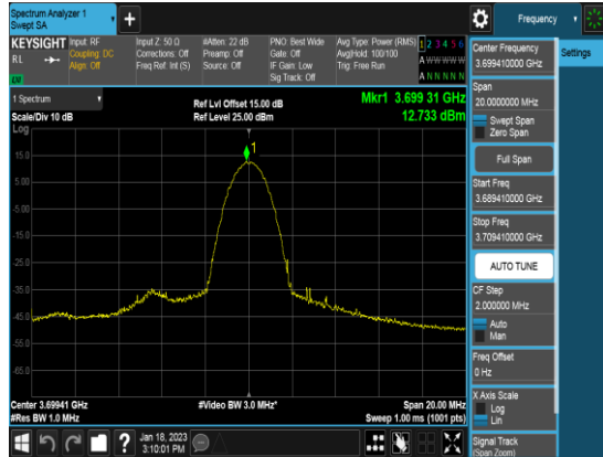
Ant 0_10M_QPSK_1RB0_PSD_Middle channel
