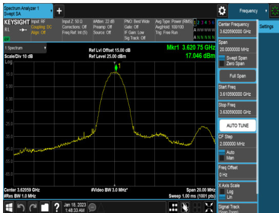
10M_Q64_FULLRB_PSD_Low channe
