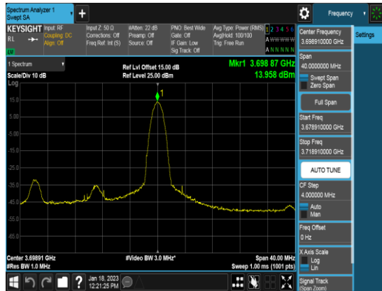
Ant 0_20M_QPSK_1RB0_PSD_Middle channel
