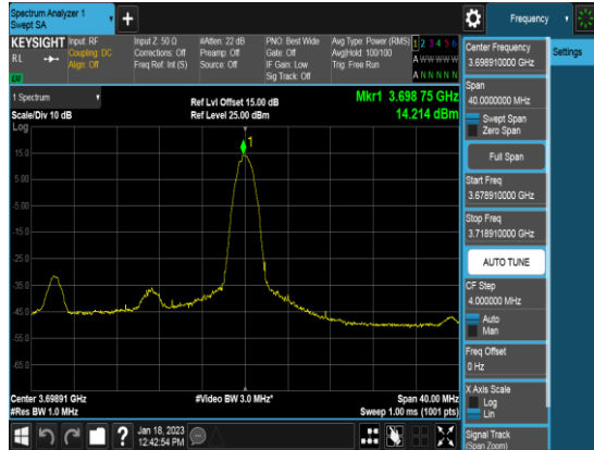
Ant 0_20M_Q64_1RB0_PSD_Middle channel
