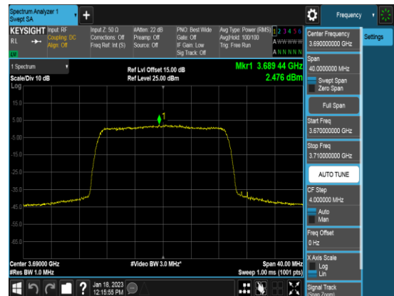
Ant 0_20M_QPSK_FULLRB_PSD_Middle channel
