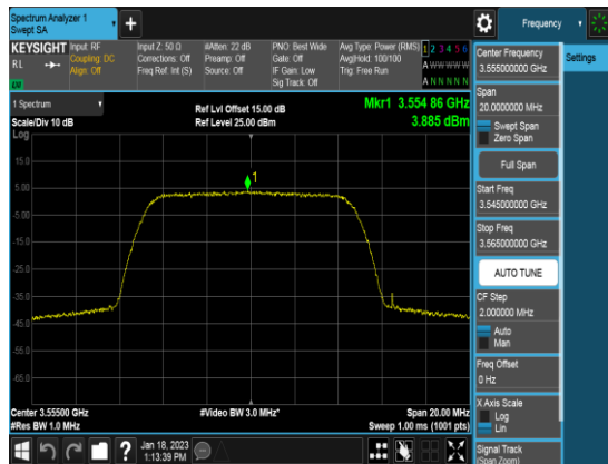
Ant 0_10M_Q64_FULLLRB_PSD_Low channel
