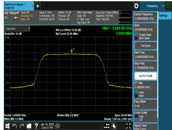
Ant 0_10M_QPSK_FULLRB_PSD_Middle channel
