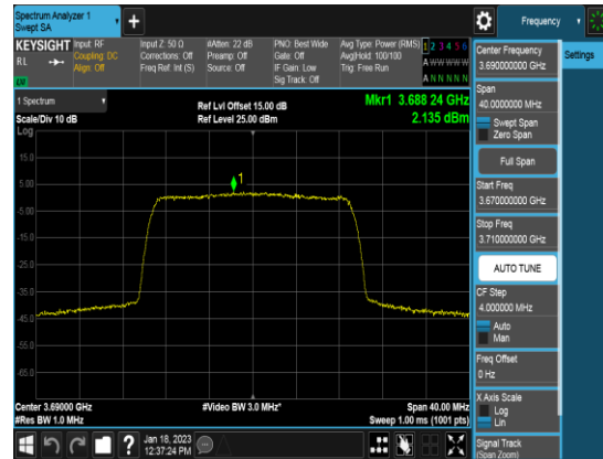
Ant 0_20M_Q64_FULLLRB_PSD_Middle channel
