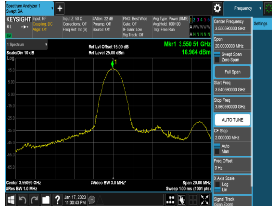
10M_Q16_FULLRB_PSD_High channel
