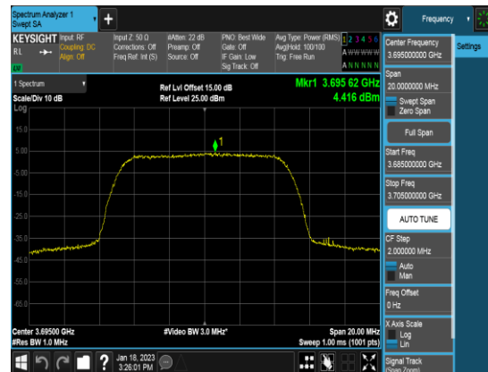
Ant 0_10M_Q64_FULLLRB_PSD_Middle channel
