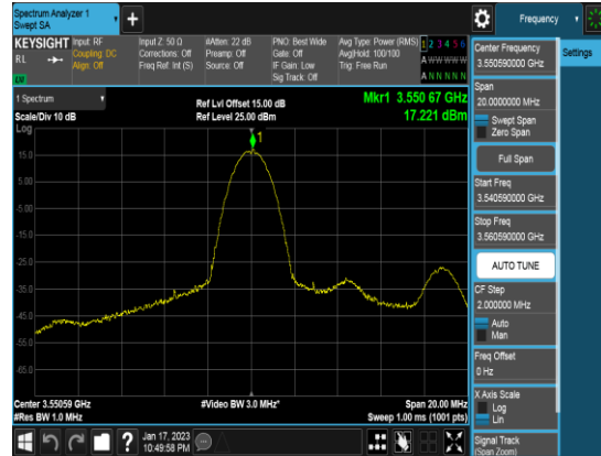
10M_QPSK_FULLRB_PSD_High channel
