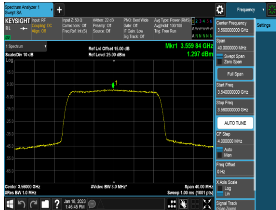
Ant 0_20M_Q64_FULLLRB_PSD_Low channel
