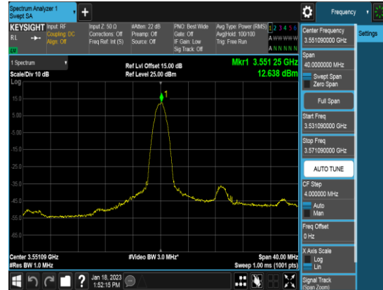
Ant 0_20M_Q64_FULLLRB_PSD_High channel
