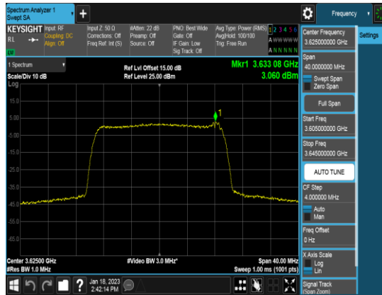
Ant 0_20M_Q16_FULLLRB_PSD_Middle channel
