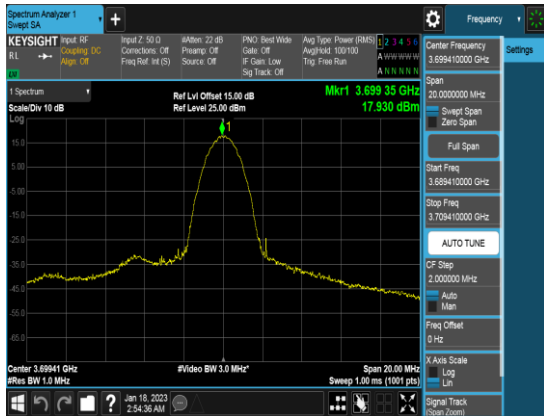
10M_Q64_1RB0_PSD_Middle channel
