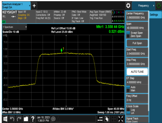
Ant 0_20M_Q16_FULLLRB_PSD_Low channel
