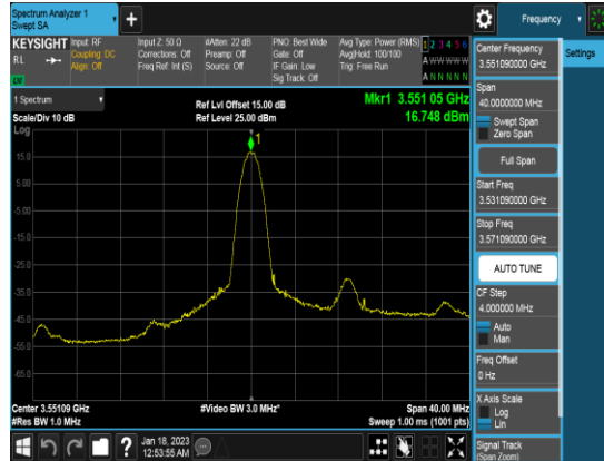
20M_QPSK_FULLRB_PSD_High channel
