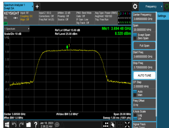
10M_Q16_FULLRB_PSD_Middle channel
