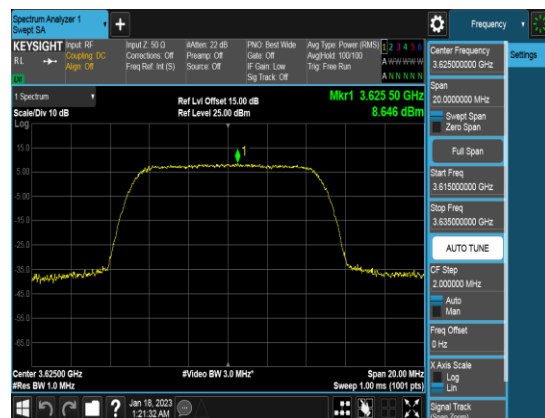
10M_QPSK_FULLRB_PSD_Middle channel
