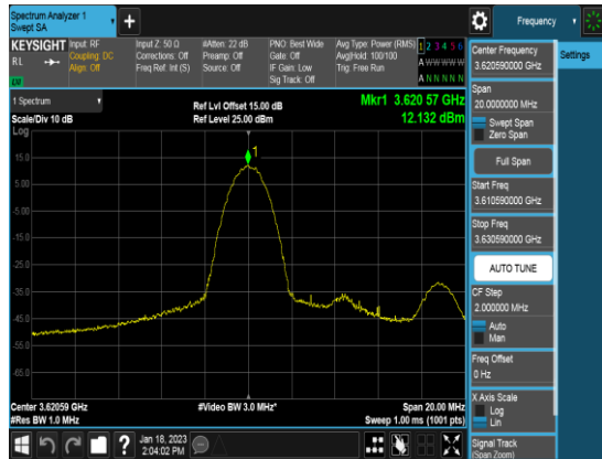
Ant 0_10M_QPSK_FULLRB_PSD_Low channel
