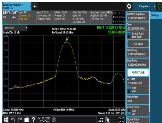
10M_Q16_FULLRB_PSD_Low channel
