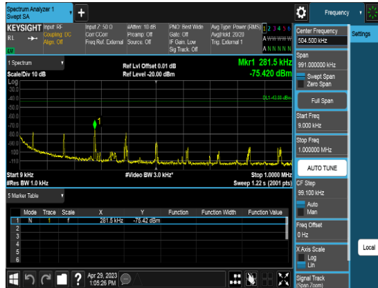
Port1_5M_3625MHz_TM3.2_CHM_CSE1
