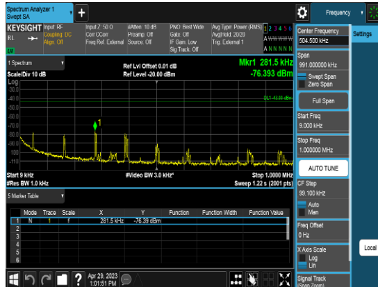
Port1_5M_3552.5MHz_TM3.2_CHL_CSE1
