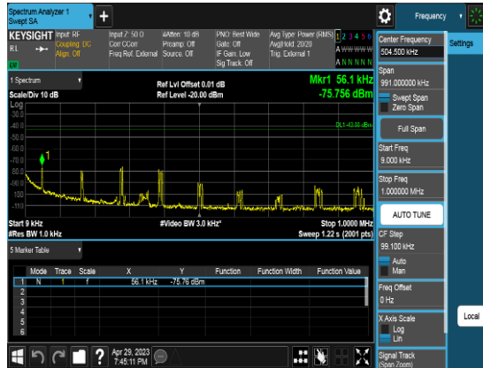
Port2_15M_3625MHz_TM3.2_CHM_CSE1
