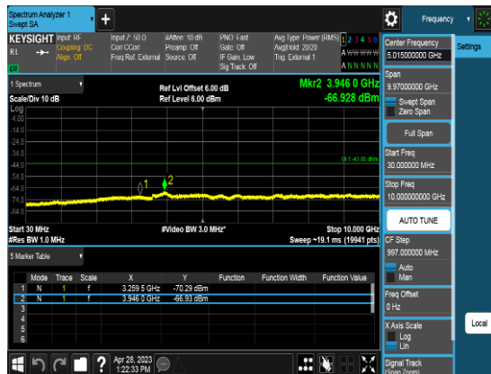
Port1_20M_3625MHz_TM3.2_CHM_CSE3
