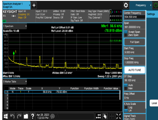
Port1_20M_3625MHz_TM3.2_CHM_CSE1
