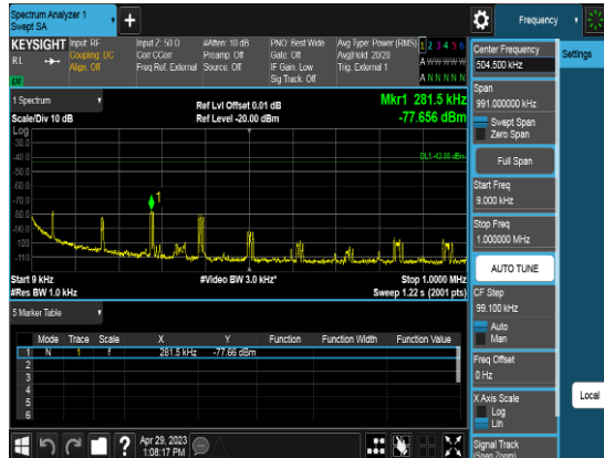
Port1_5M_3697.5MHz_TM3.2_CHH_CSE1
