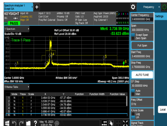
Port1_5M_3552.5MHz_TM3.2_CHL_CSEpart96
