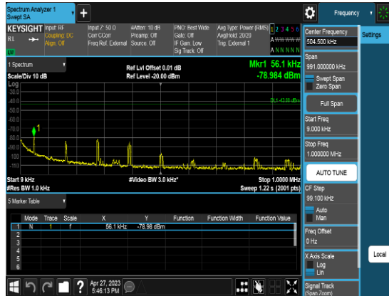
Port2_10M_3695MHz_TM3.2_CHH_CSE1
