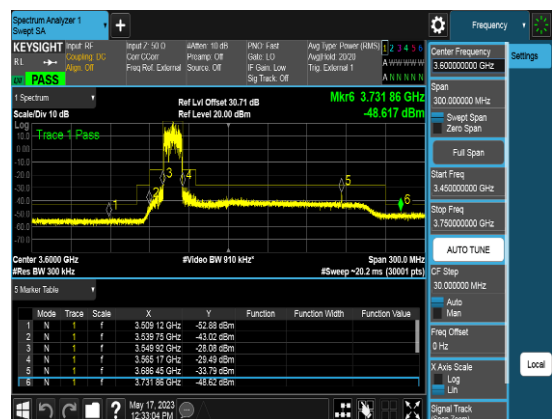
Port2_15M_3557.5MHz_TM3.2_CHL_CSEpart96
