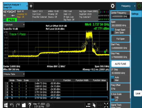
Port1_20M_3690MHz_TM3.2_CHH_CSEpart96
