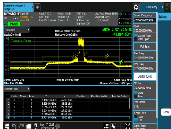
Port2_15M_3625MHz_TM3.2_CHM_CSEpart96
