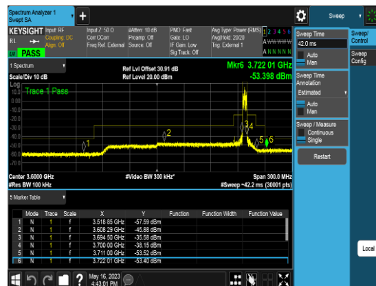
Port1_5M_3697.5MHz_TM3.2_CHH_CSEpart96
