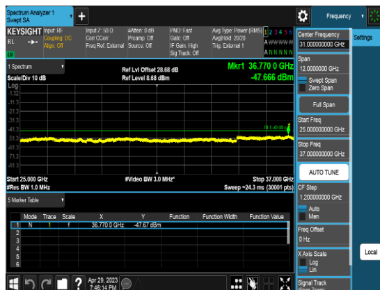
Port2_15M_3625MHz_TM3.2_CHM_CSE3
