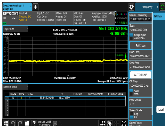
Port1_5M_3697.5MHz_TM3.2_CHH_CSE3
