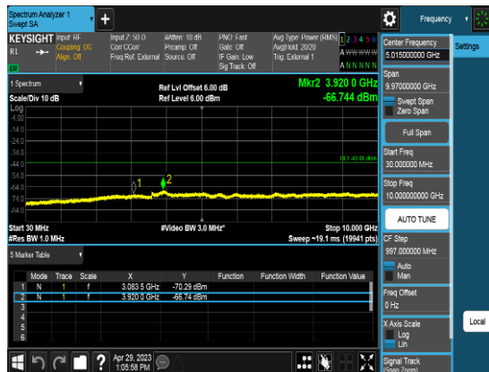
Port1_5M_3625MHz_TM3.2_CHM_CSE3
