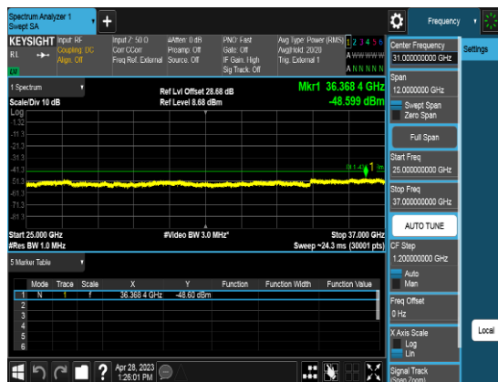
Port1_20M_3690MHz_TM3.2_CHH_CSE3
