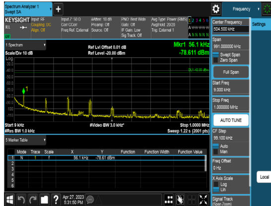
Port2_10M_3555MHz_TM3.2_CHL_CSE1
