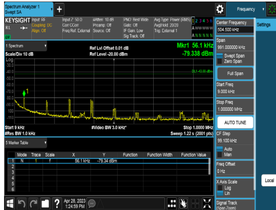
Port1_20M_3690MHz_TM3.2_CHH_CSE1
