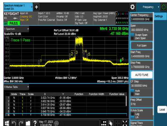
Port1_20M_3625MHz_TM3.2_CHM_CSEpart96
