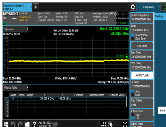
Port2_5M_3552.5MHz_TM1.1_CHL_CSE3
