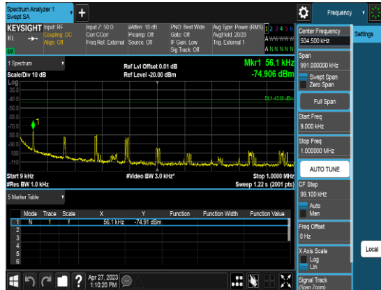
Port1_10M_3555MHz_TM3.1_CHL_CSE1
