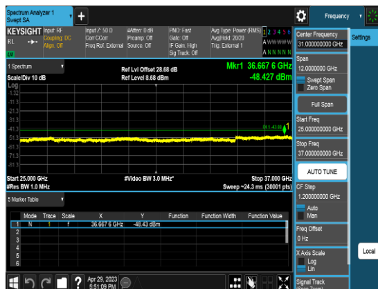
Port1_15M_3692.5MHz_TM3.1_CHH_CSE3
