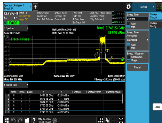
Port1_15M_3692.5MHz_TM3.1_CHH_CSEpart96
