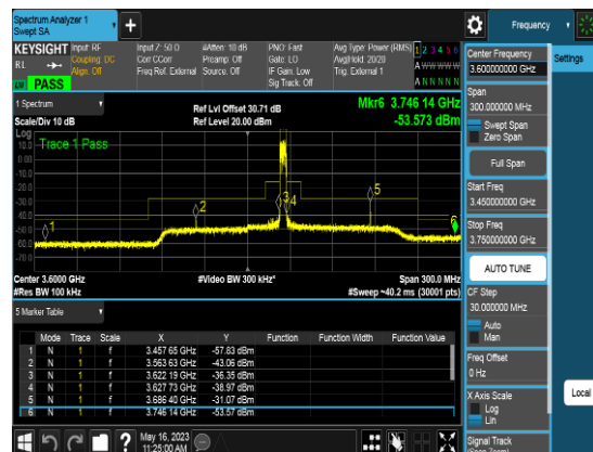
Port2_5M_3625MHz_TM1.1_CHM_CSEpart96
