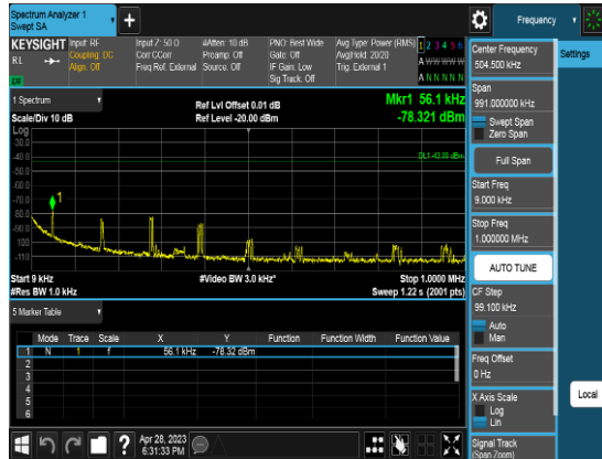
Port2_5M_3697.5MHz_TM1.1_CHH_CSE1
