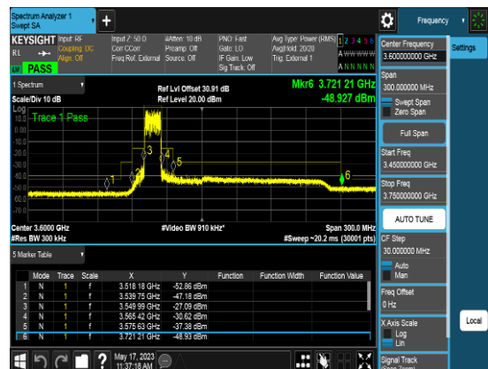
Port1_15M_3557.5MHz_TM3.1_CHL_CSEpart96
