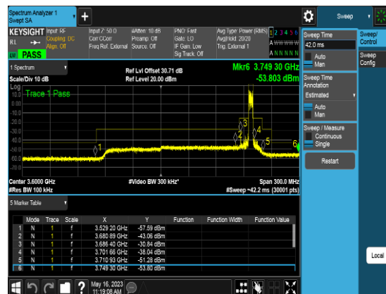
Port2_5M_3697.5MHz_TM1.1_CHH_CSEpart96
