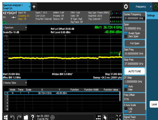
Port1_15M_3557.5MHz_TM3.1_CHL_CSE3
