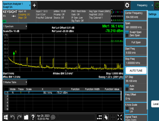
Port2_5M_3552.5MHz_TM1.1_CHL_CSE1
