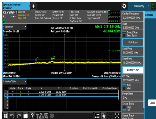
Port2_5M_3697.5MHz_TM1.1_CHH_CSE3
