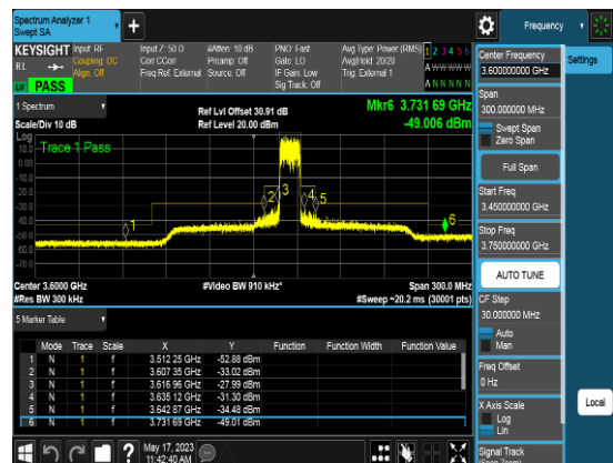
Port1_15M_3625MHz_TM3.1_CHM_CSEpart96
