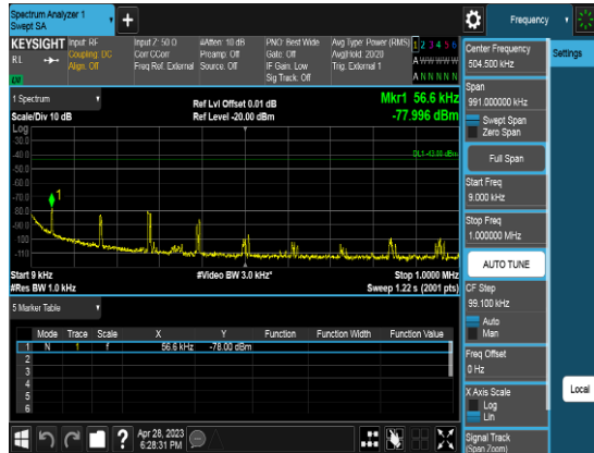
Port2_5M_3625MHz_TM1.1_CHM_CSE1
