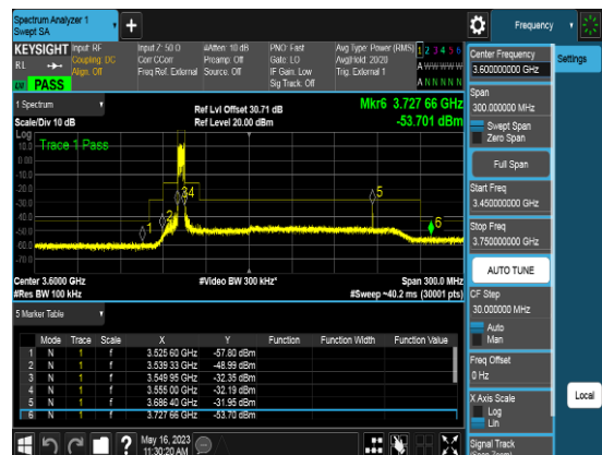
Port2_5M_3552.5MHz_TM1.1_CHL_CSEpart96
