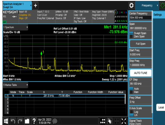
Port1_15M_3692.5MHz_TM3.1_CHH_CSE1
