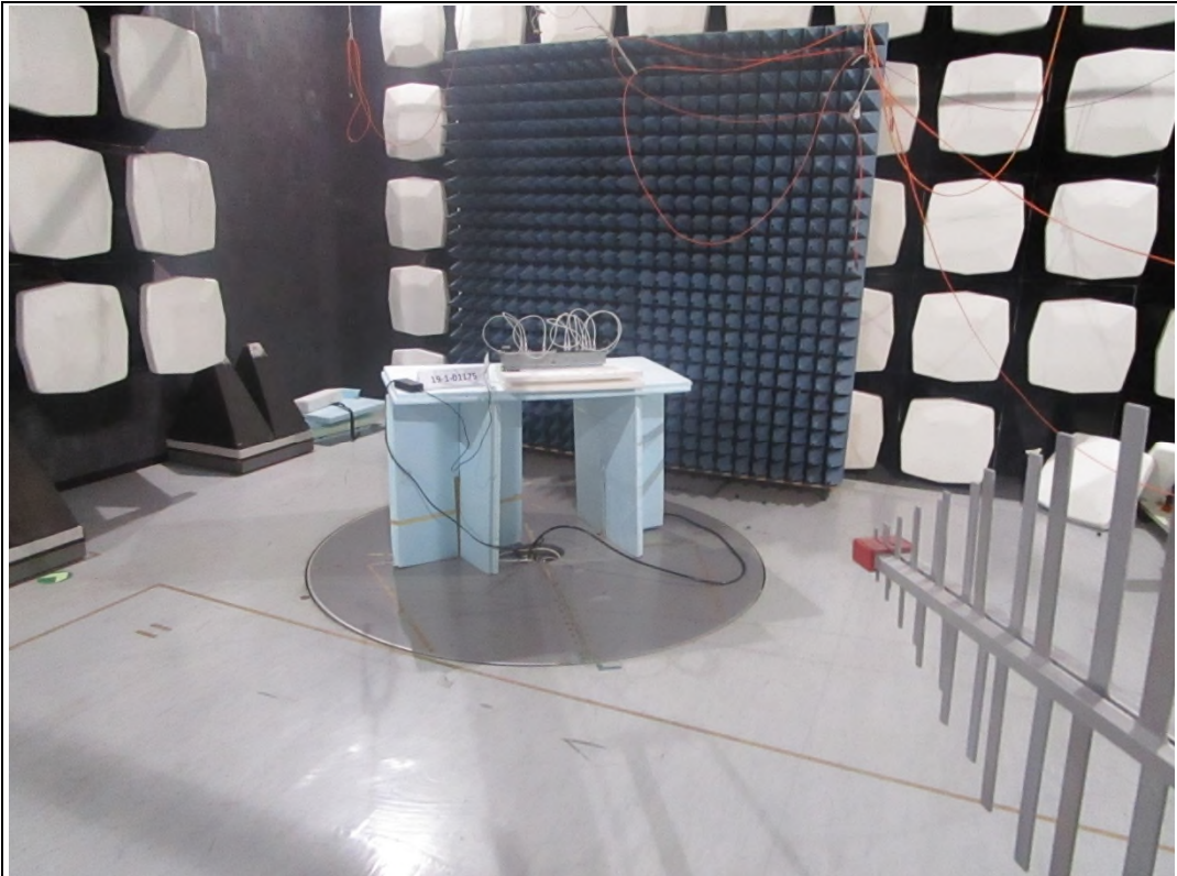
Photograph 5: Test set-up
