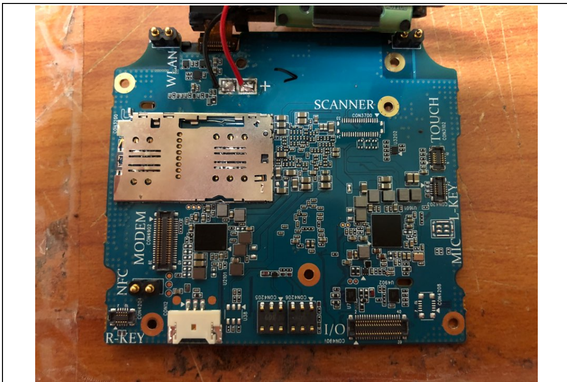
MainBoard-Rear
