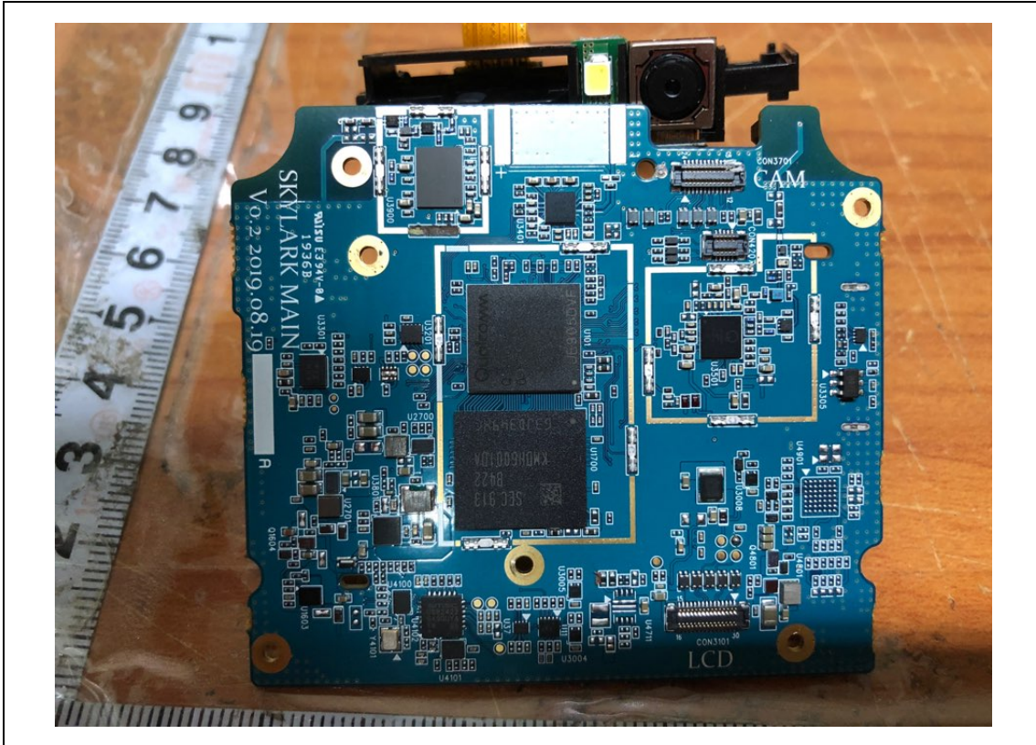
MainBoard-Rear
