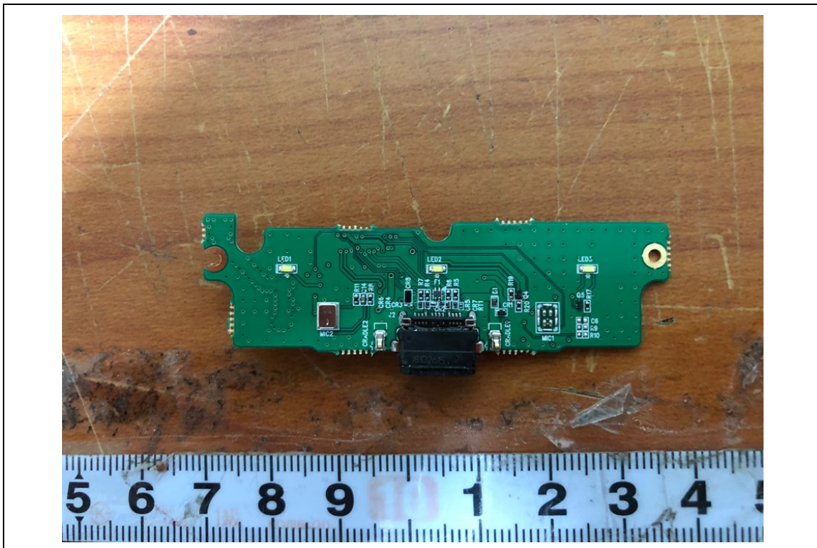
Module Board-Rear
