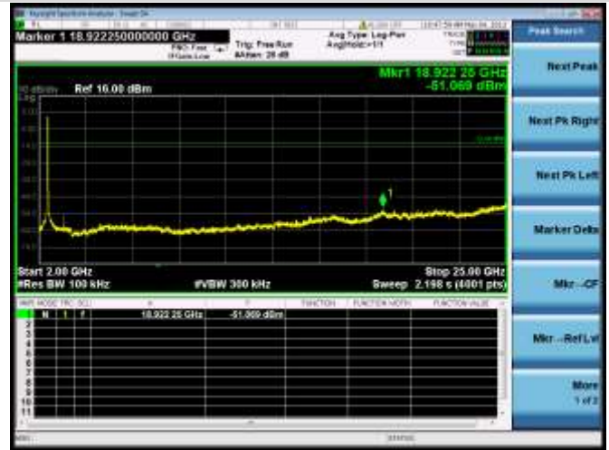
802.11n-20 MHz MIDDLE CHANNEL, SPURIOUS 2 GHz ~ 25 GHz
