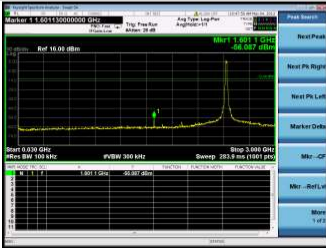
802.11n-20 MHz MIDDLE CHANNEL, SPURIOUS 30 MHz ~ 3 GHz
