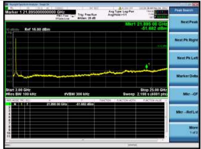
802.11g MIDDLE CHANNEL, SPURIOUS 2 GHz ~ 25 GHz
