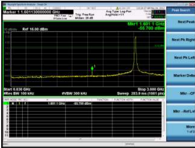
802.11g MIDDLE CHANNEL, SPURIOUS 30 MHz ~ 3 GHz
