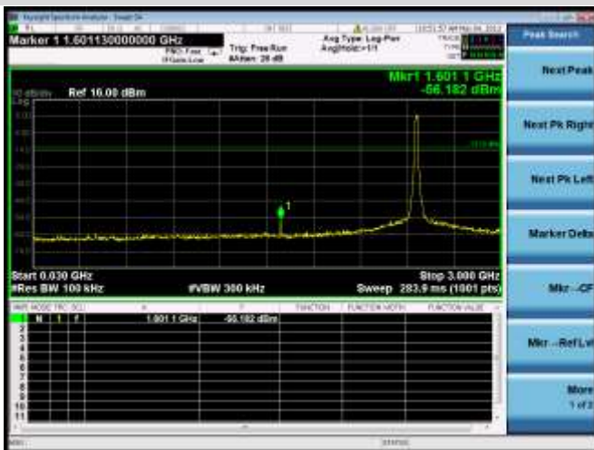
802.11n-20 MHz HIGH CHANNEL, SPURIOUS 30 MHz ~ 3 GHz
