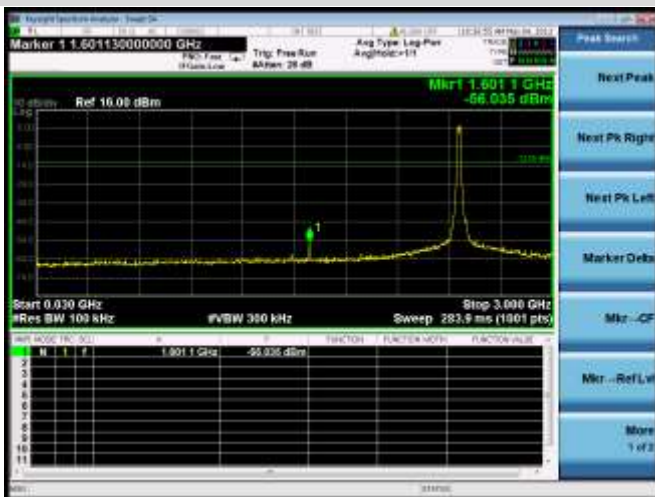
802.11g HIGH CHANNEL, SPURIOUS 30 MHz ~ 3 GHz
