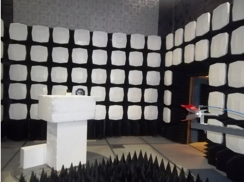
Figure 10: Equipment Under Test – Radiated Emissions >1GHz
