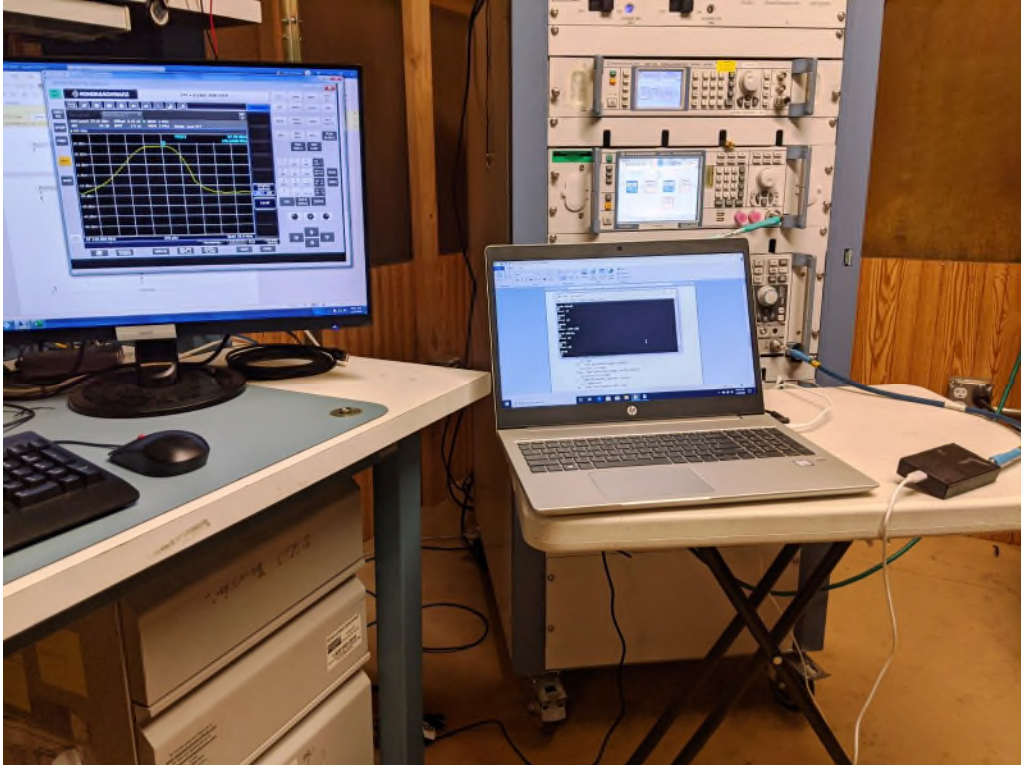
Figure 2: Equipment Under Test – Antenna Port Conducted Measurements (Licensed)
