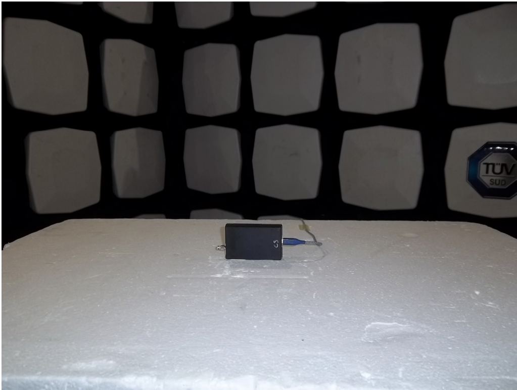
Figure 3: Equipment Under Test – Radiated Emissions – X-orientation
