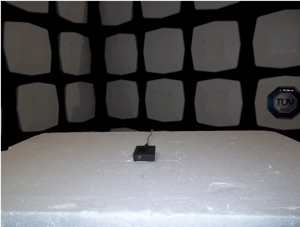
Figure 5: Equipment Under Test – Radiated Emissions Z-orientation
