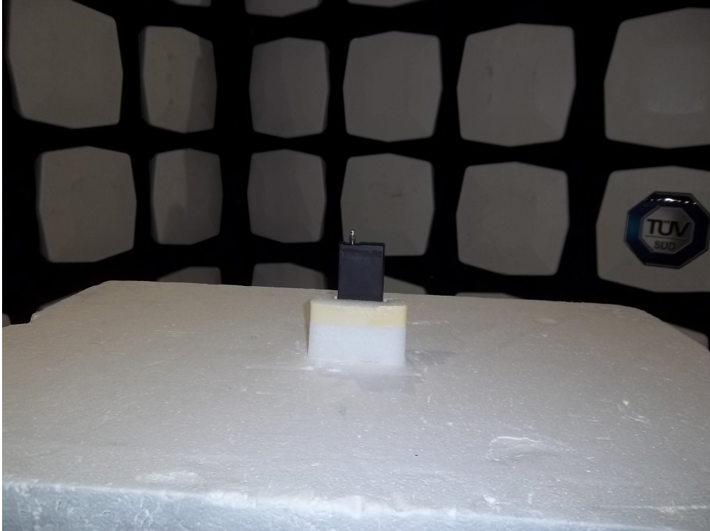
Figure 4: Equipment Under Test – Radiated Emissions – Y-orientation
