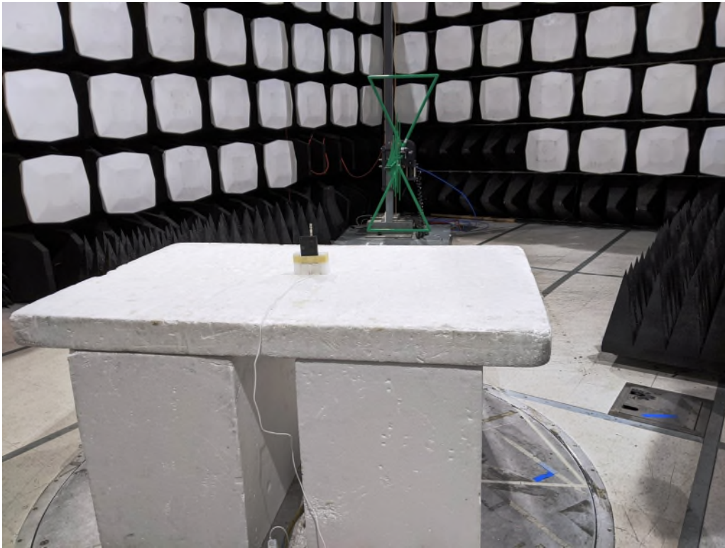
Figure 9: Equipment Under Test – Radiated Emissions <1GHz
