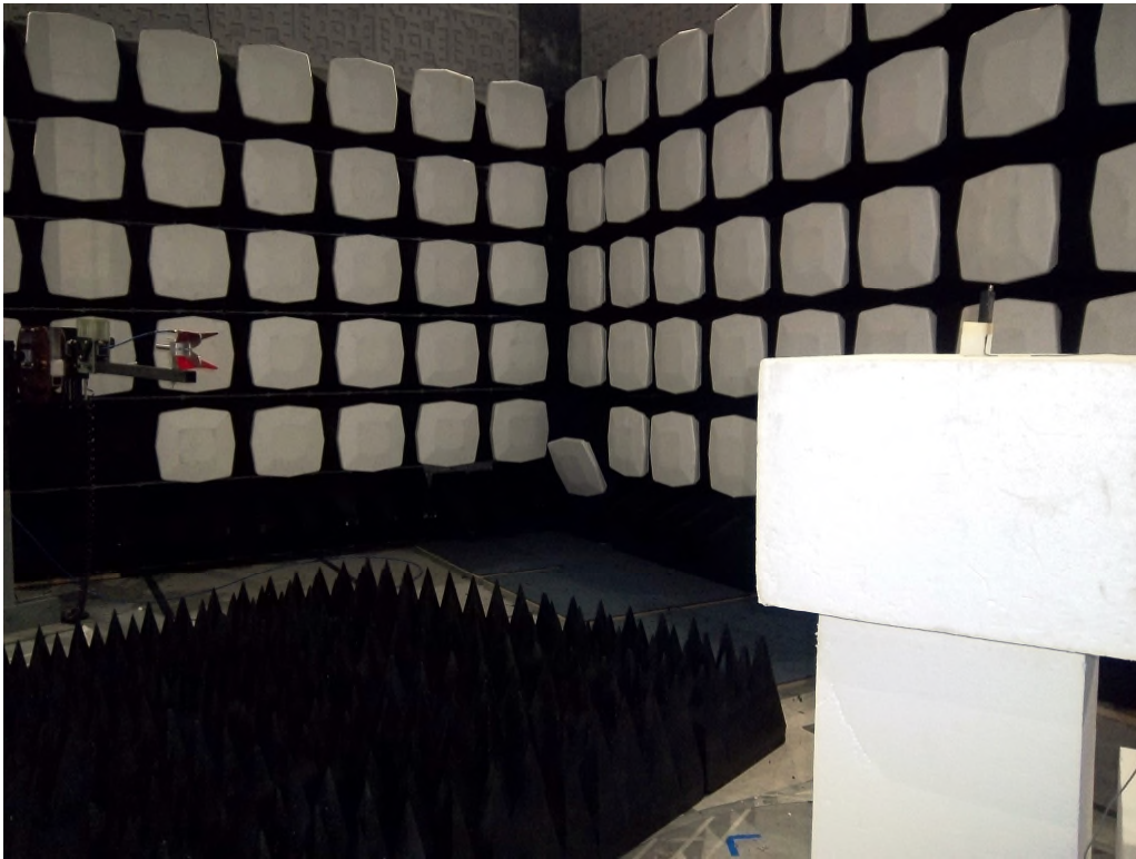
Figure 11: Equipment Under Test – Radiated Emissions >1GHz
