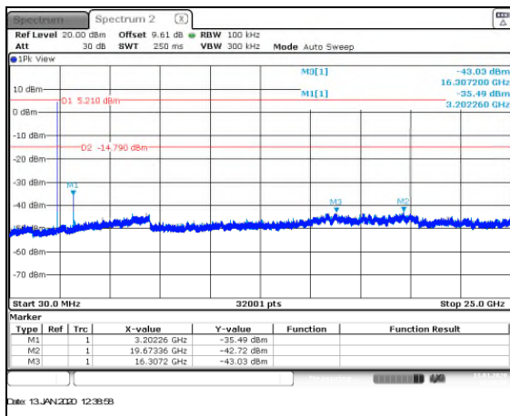
Figure 7.5.1.2-1: LCH – 30MHz–25GHz
