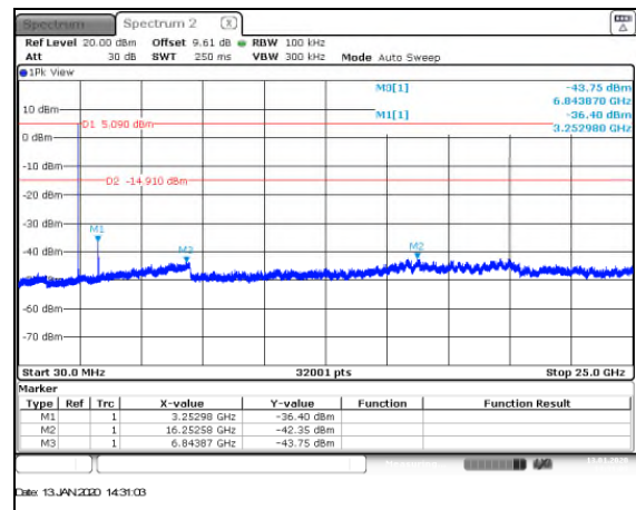
Figure 7.5.1.2-2: MCH – 30MHz–25GHz
