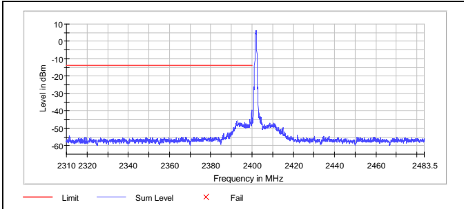
Figure 7.5.1.2-4: Lower Band-edge
