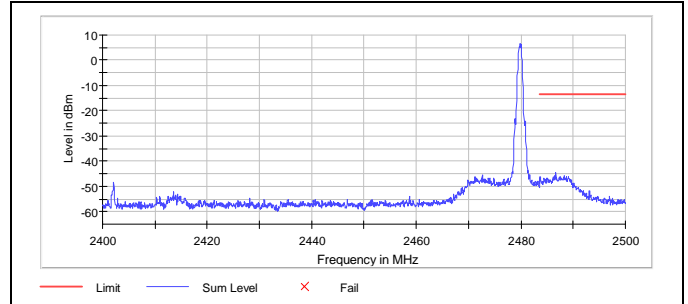
Figure 7.5.1.2-5: Upper Band-edge
