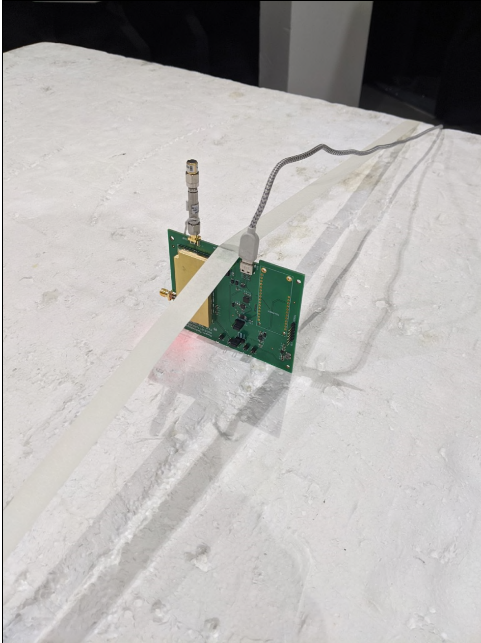
Figure 3: Equipment Under Test – Radiated Emissions – Y-orientation
