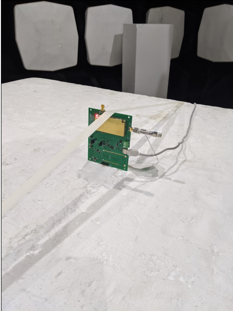
Figure 2: Equipment Under Test – Radiated Emissions – X-orientation
