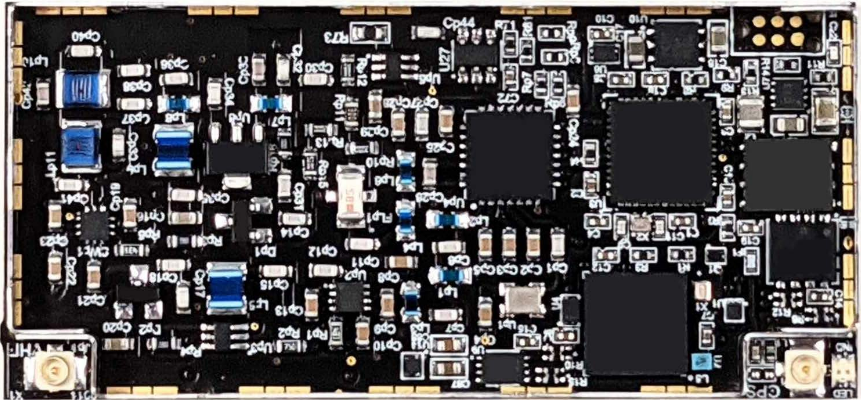
Figure 1: Top View
