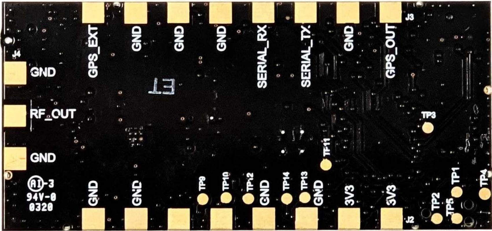
Figure 2: Bottom View
