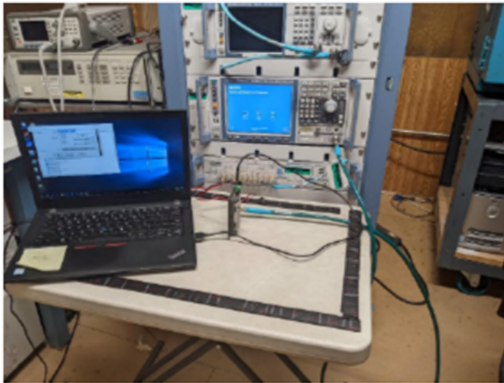
Figure A-4 – Test Set up – Antenna Port measurements
