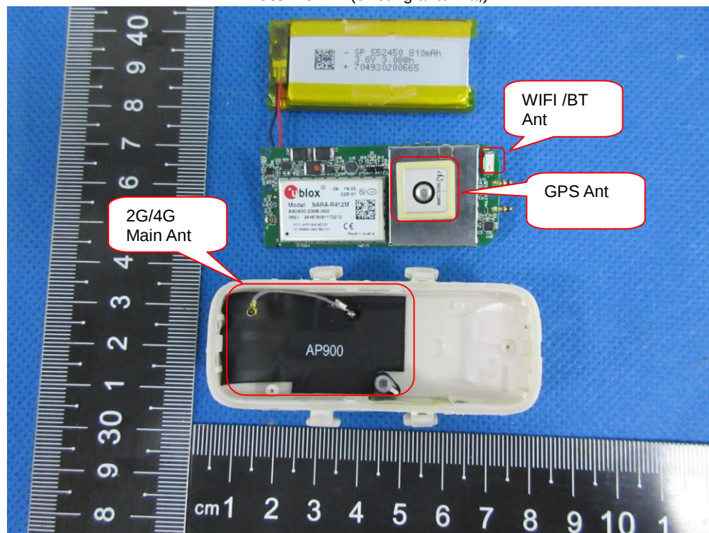
Photo 10 (existing antenna,)
