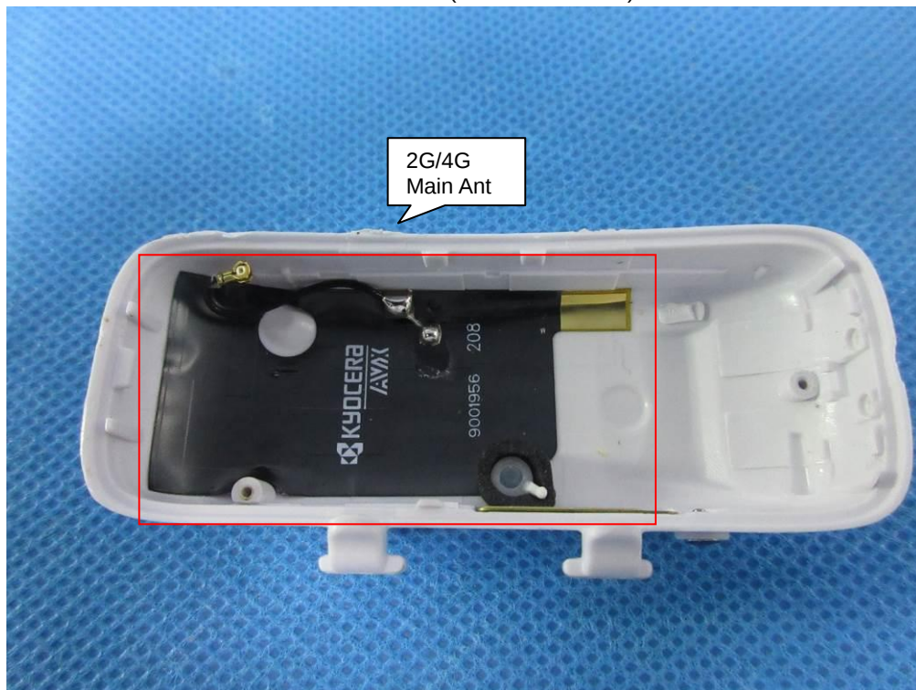
Photo 11 (alternate antenna)
