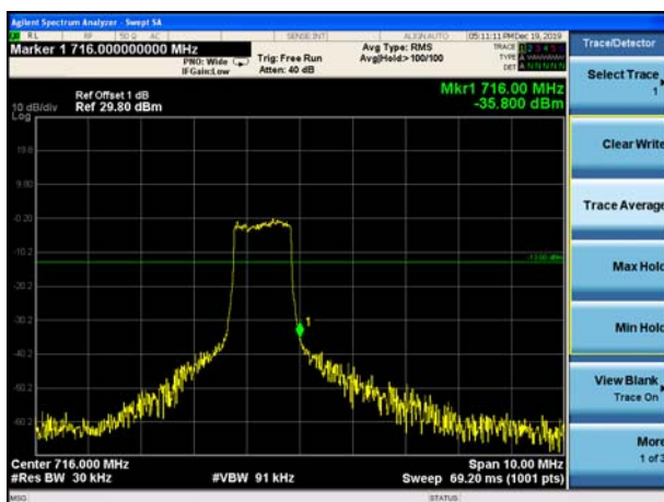
CAT M1 B12 QPSK BW 1.4, NO. RB 6,CH-High
