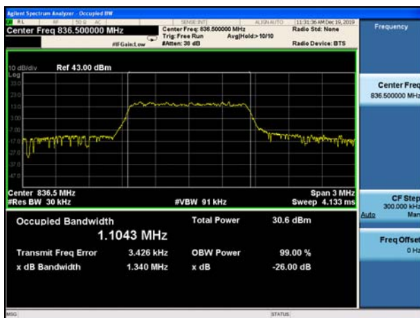
CAT M1 B5 QPSK Mid Channel
