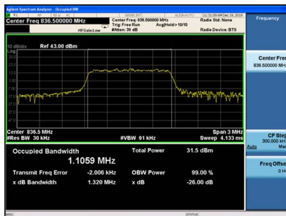
CAT M1 B5 16QAM Mid Channel
