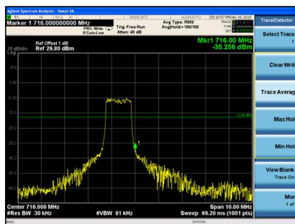
CAT M1 B12 16QAM BW 1.4, NO. RB 6,CH- High
