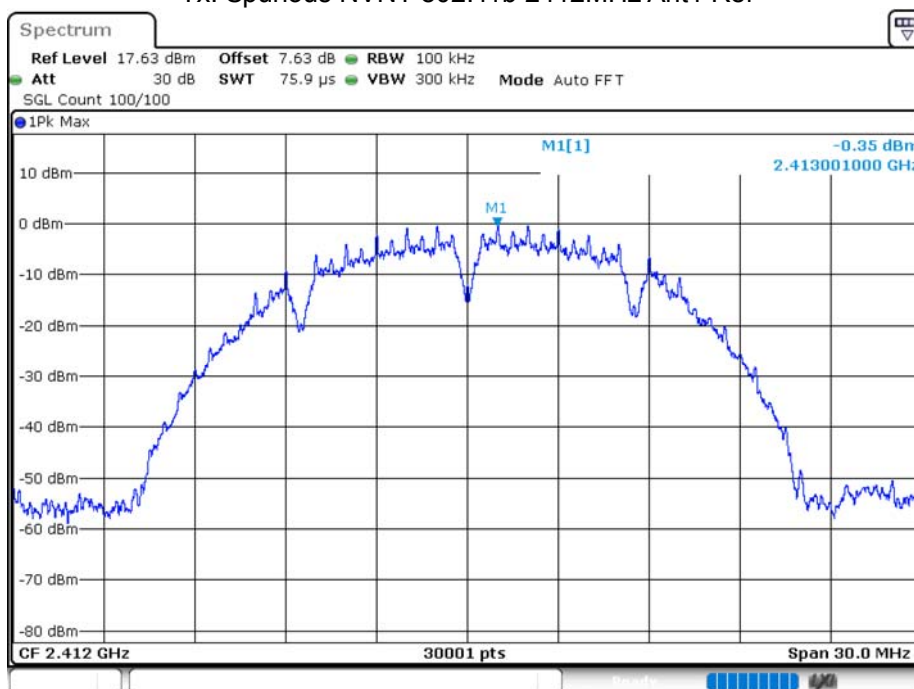
Tx. Spurious NVNT 802.11b 2412MHz Ant1 Emission
