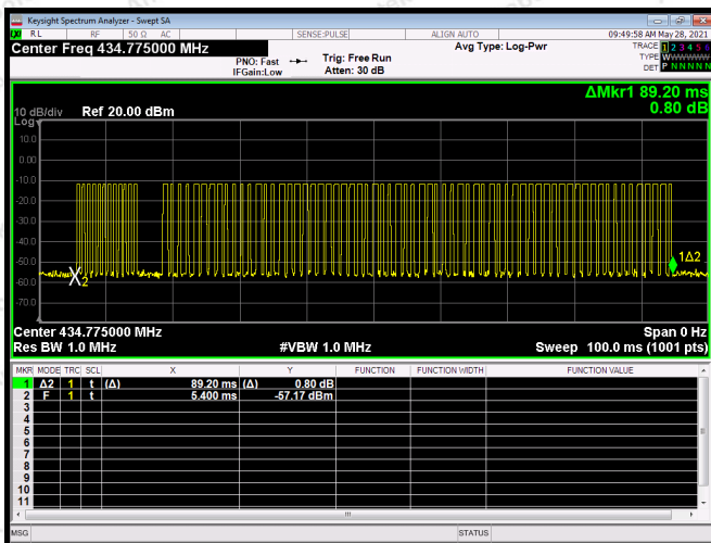
434.775MHz-T period
