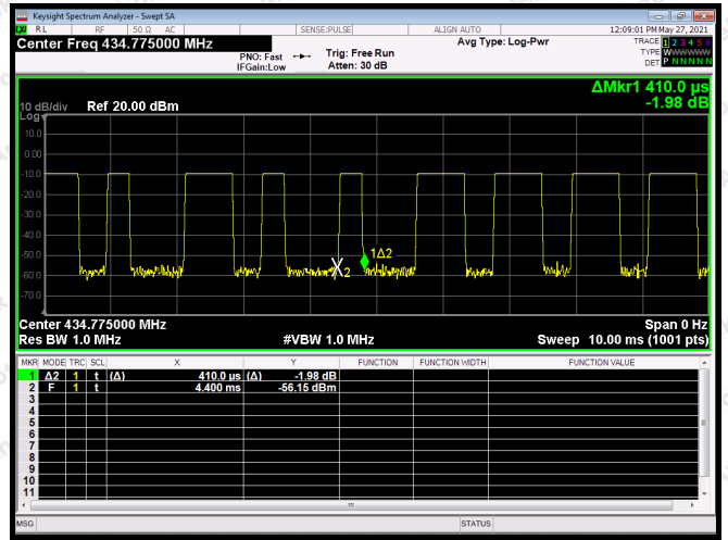
434.775MHz-T on2
