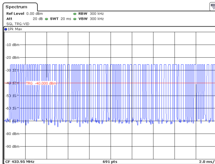
1 pulse train has 50 single small bursts and 23 single big bursts
