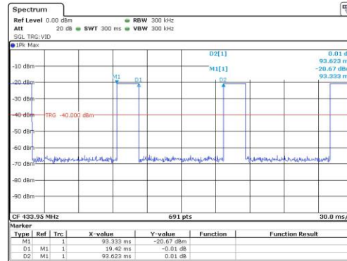
Observation period 2 (Single pulse cycle is 93.623ms)
