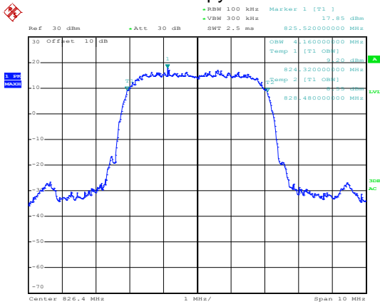
99% Occupy bandwidth
