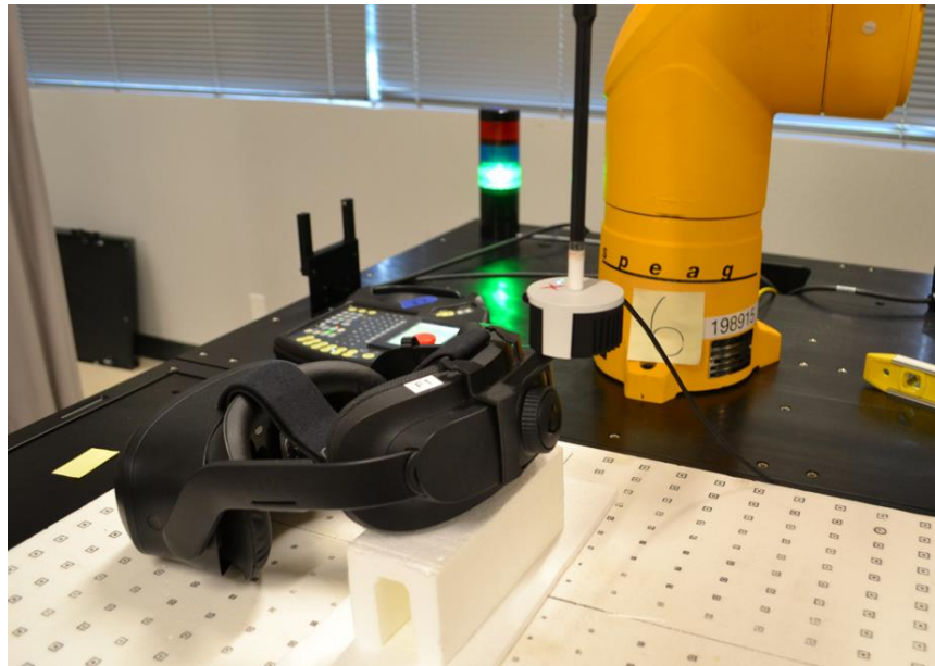
Figure 2 – Top Measurements
