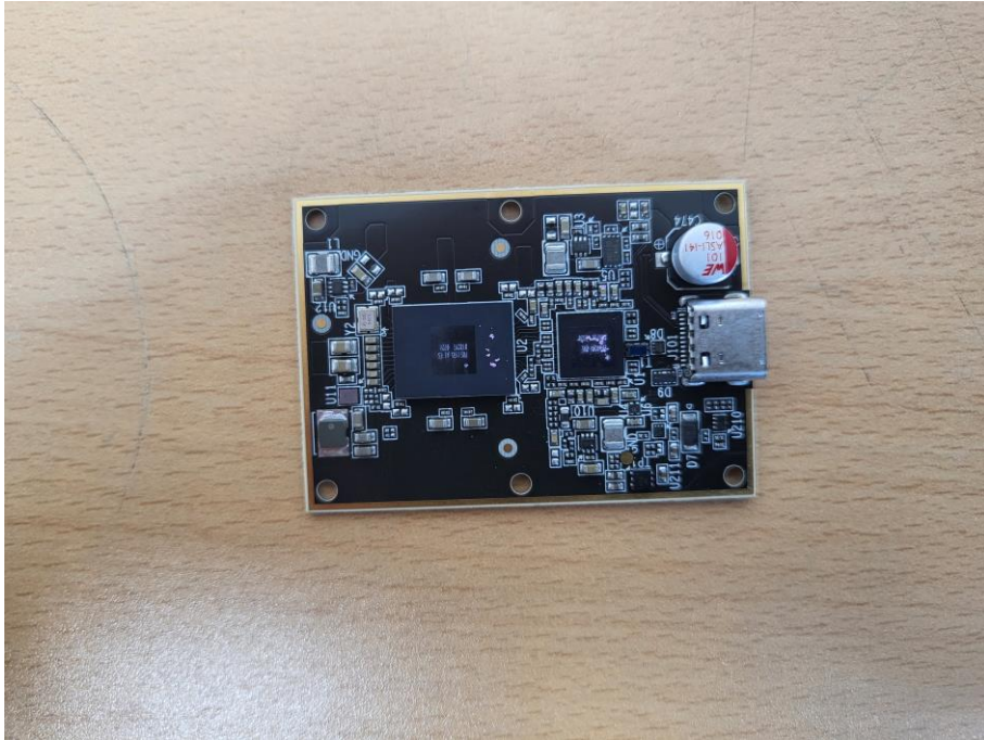
Rear View of Sub Board
