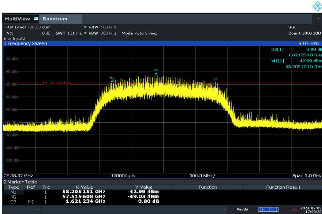
6 dB Bandwidth
