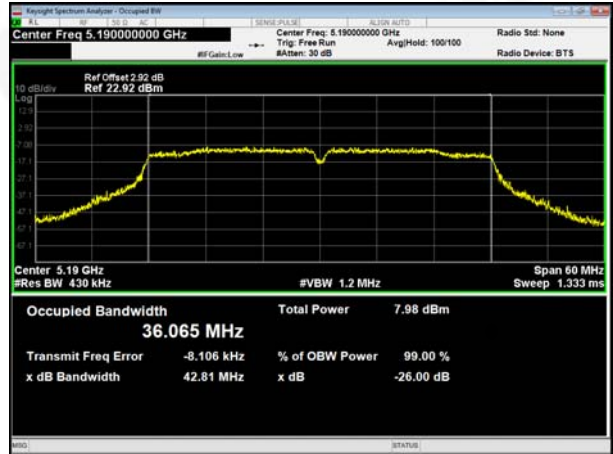
(802.11 ac40) 26dB Bandwidth plot on channel 38
