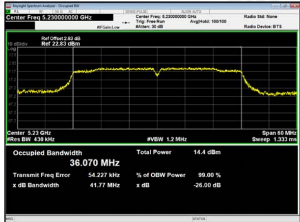
(802.11 ac40) 99% Bandwidth plot on channel 46
